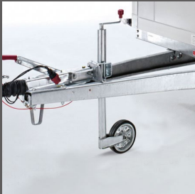
Long drawbar (version depends on model)
