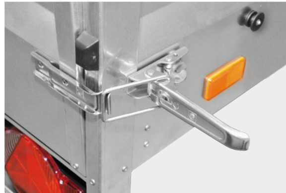
Toggle-type fasteners on the tailgate
