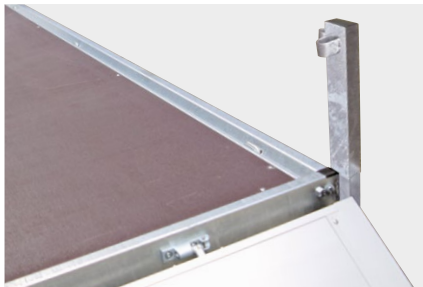
Stanchion pockets and removable stanchions, both hot-dip galvanised
