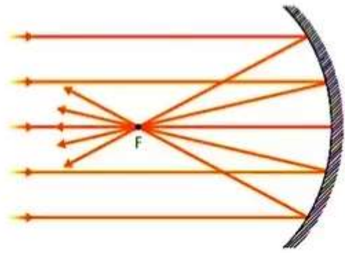
"converging" mirror
