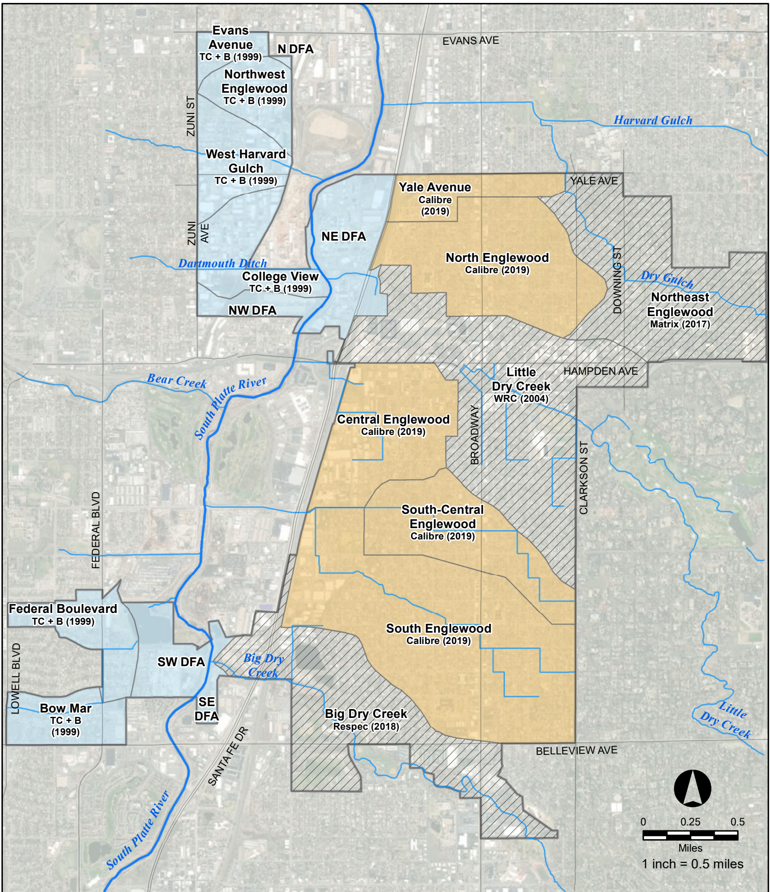
FIGURE 1 RECOMMENDED LIMITS OF STUDY FOR HYDROLOGY
