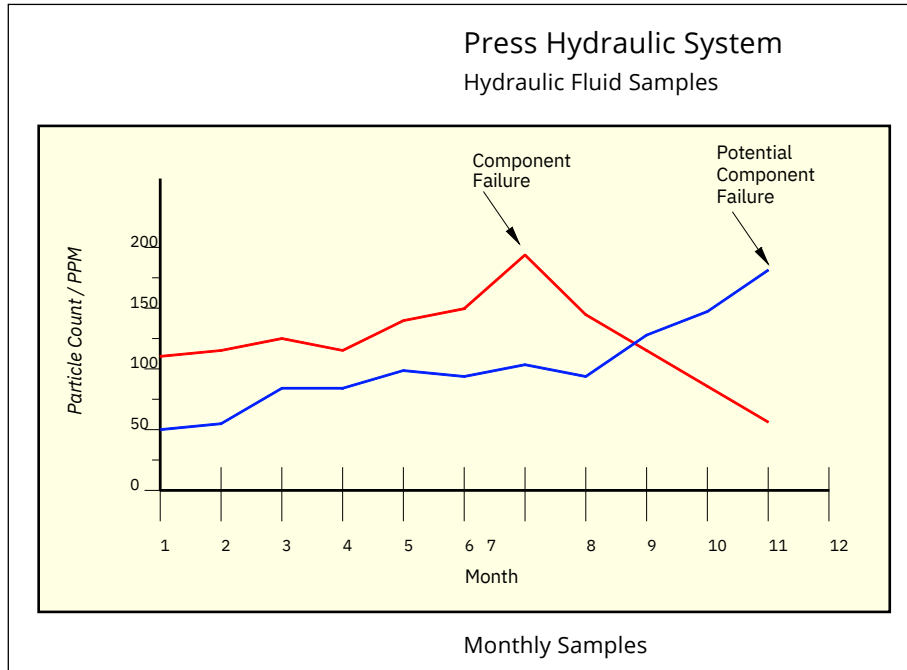
Figure 3. Hydraulic Fluid Samples
