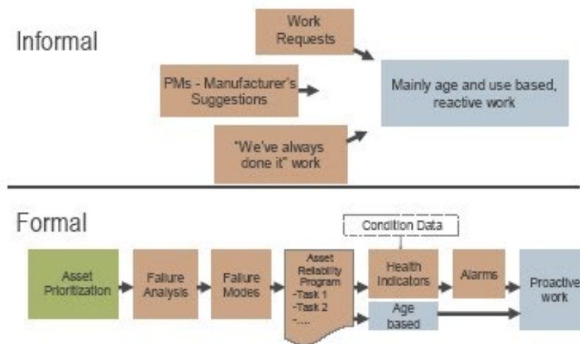
Figure 1: Progressive plants use a formal process where work orders can be traced back to the failure analysis that found the problem and created the task.
