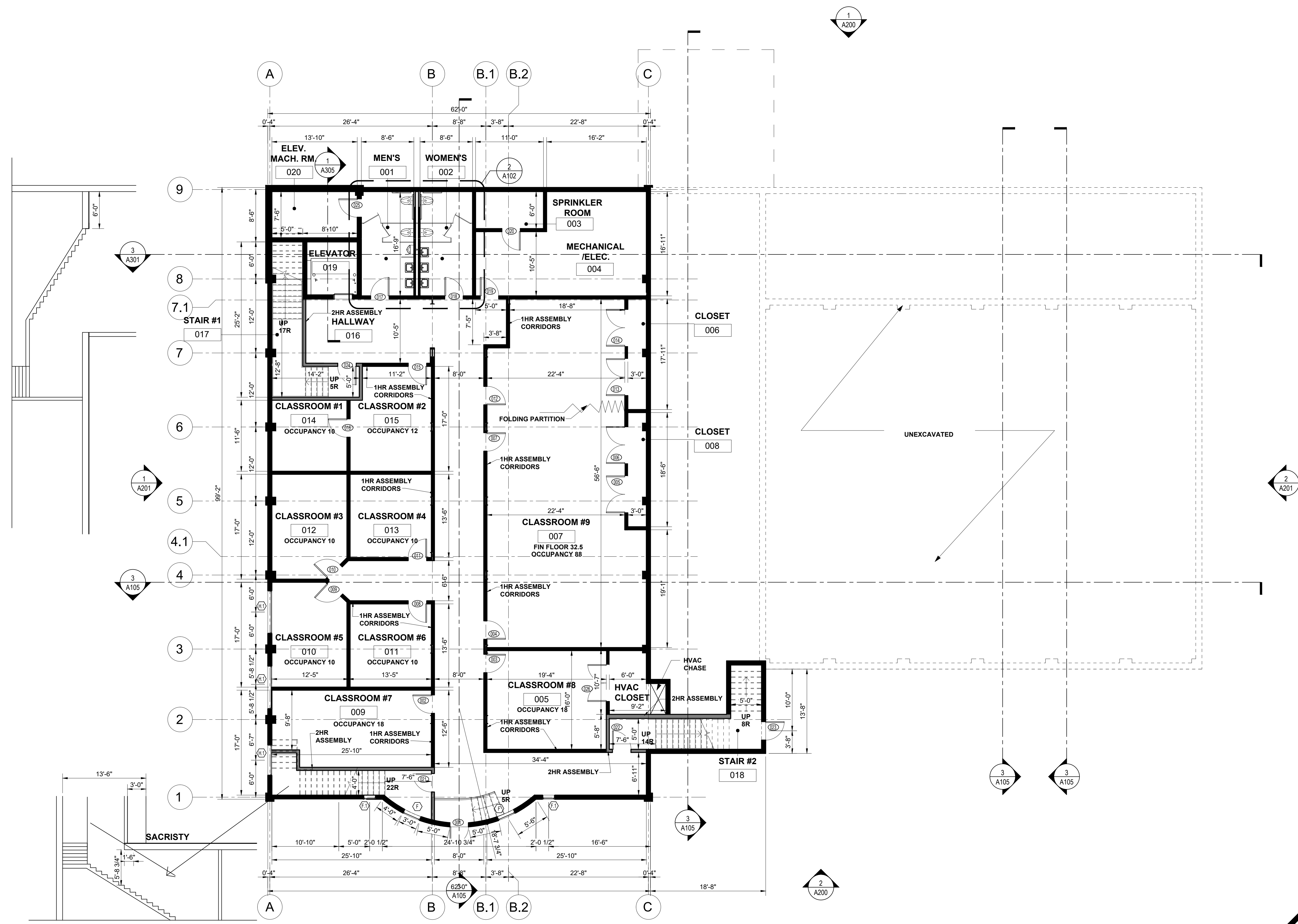
1 BASEMENT PLAN 1/8" = 1'-0"
