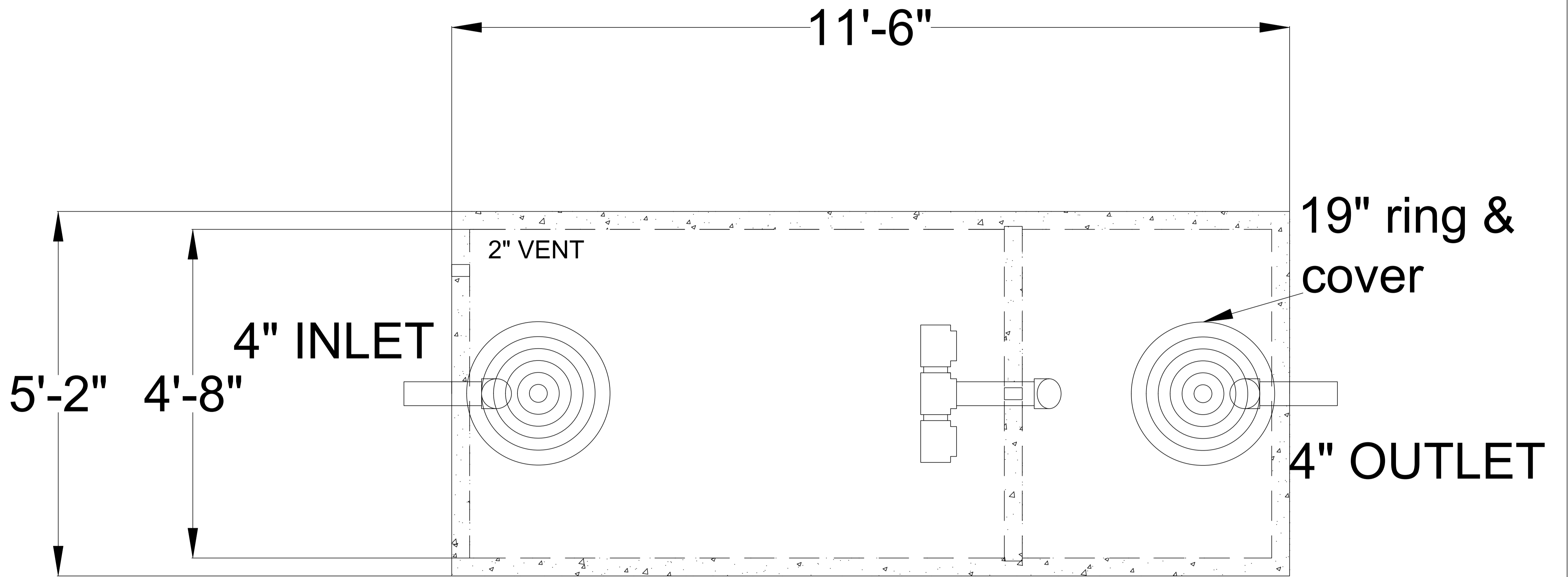
TOP VIEW
