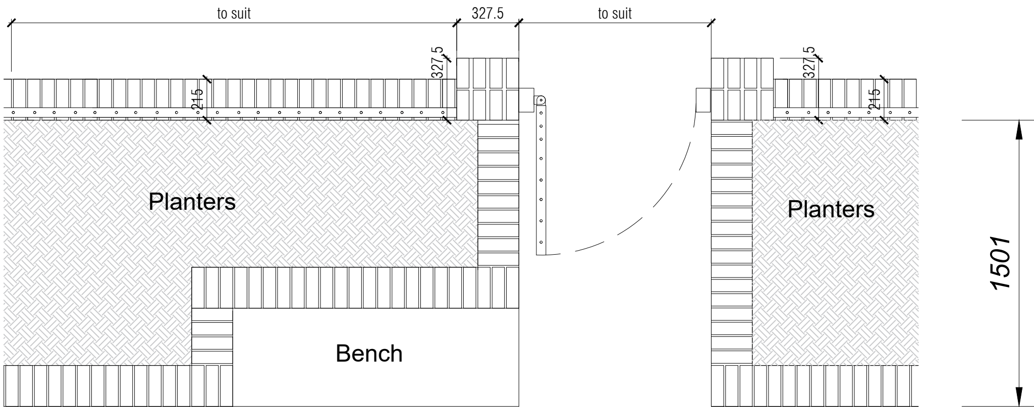
Dwarf wall with galvanised railings to front garden boundary Ref. 22007 (05) 101 - Proposed Site Layout
