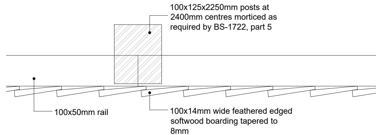
Section Detail
