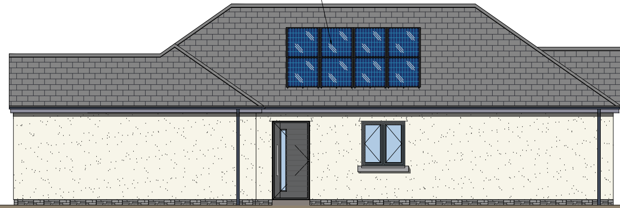
Side Elevation
