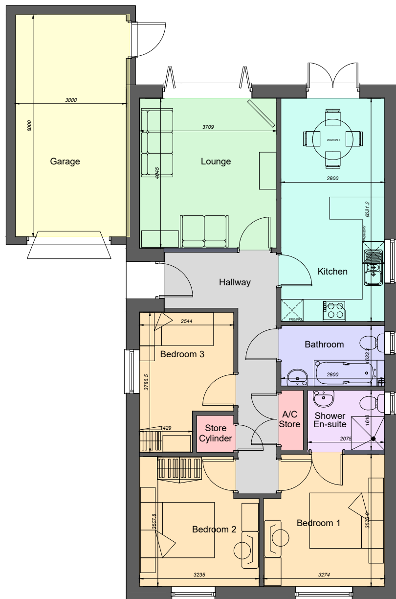
Floor Plan
