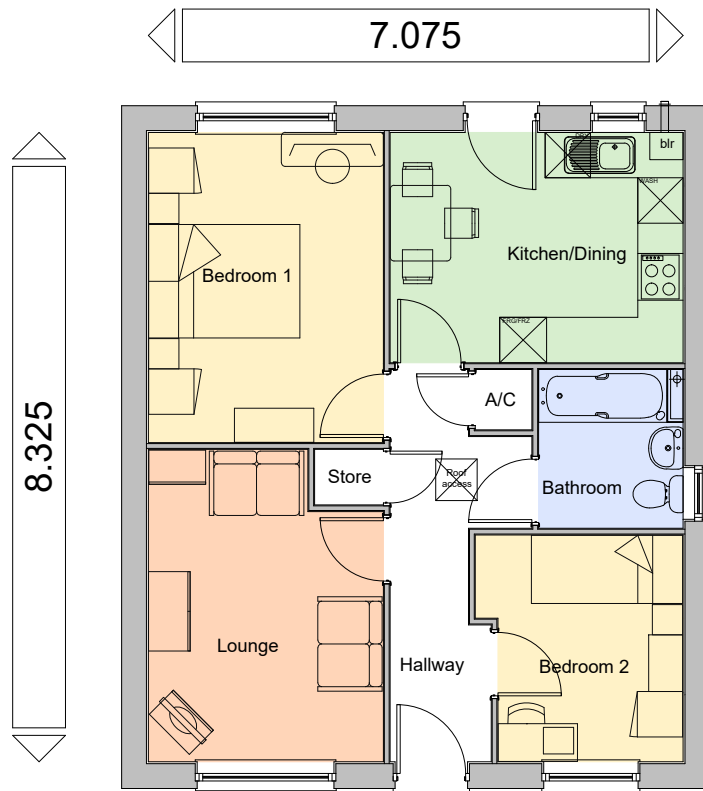
FLOOR PLAN
