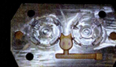
Harris Pattern
