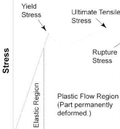
Stress Strain Curve Steel
