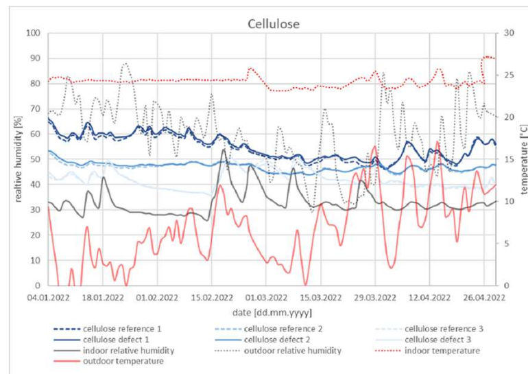
Fischer H and Korjenic A (2023) Hygrothermal Performance of Bio-Based Exterior Wall Constructions and Their Resilience under Air Leakage and Moisture Load. Buildings 2023, 13, 2650.
