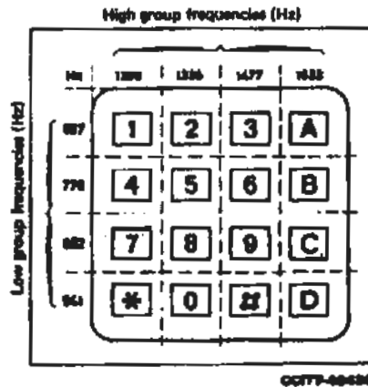
FIGURE 1/Q.23 Allocation of frequencies to the various digits and symbols of a push-button set
