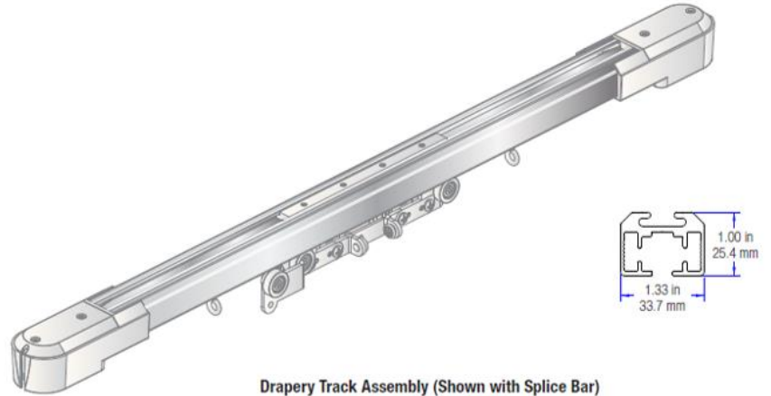
Drapery Track Assembly (Shown with Splice Bar) (CSA-DRP-TRACK-ASM)
