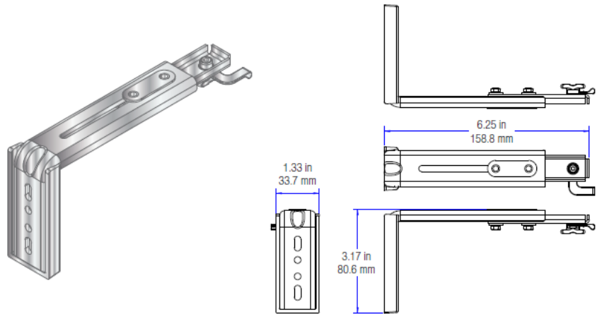
Mounting Bracket, Single (Qty. 2) (CSA-DRP-BRKT)
