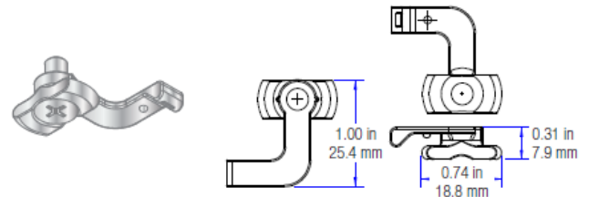
Cam Lock Mounting Bracket (Qty. 2) (CSA-DRP-CAM-LOCK)
