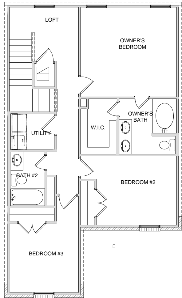
SECOND FLOOR
