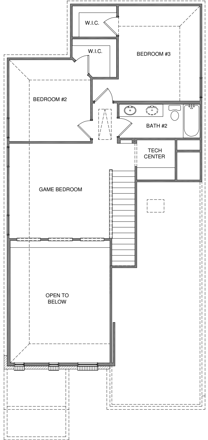
SECOND FLOOR
