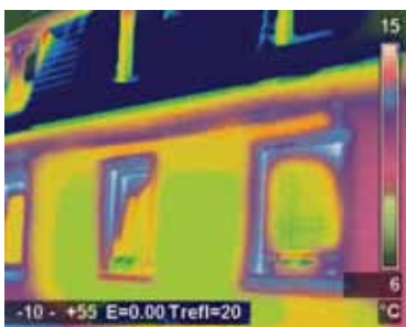
Red areas have been eliminated after fitting energy efficient windows.
