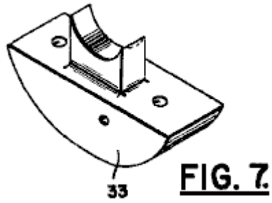
Fig.7. Shows an enlarged view of the pendulum:
