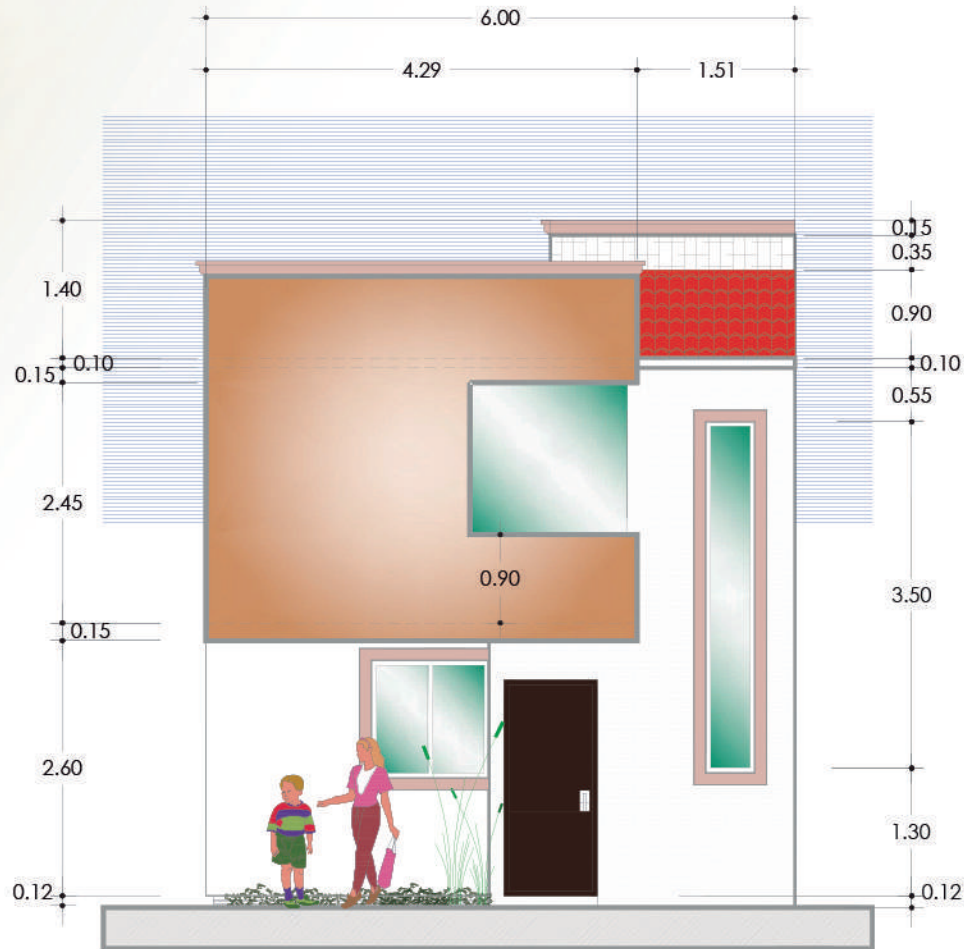
FACHADA PRINCIPAL
