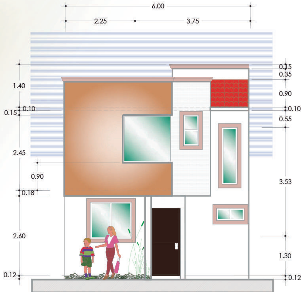
FACHADA PRINCIPAL
