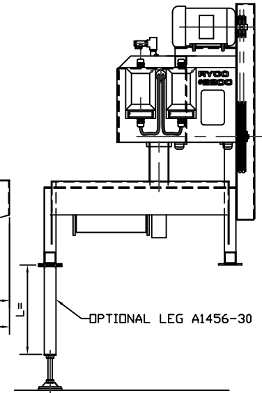
INFEEED ELEVATION
