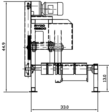
OUTFEED ELEVATION
