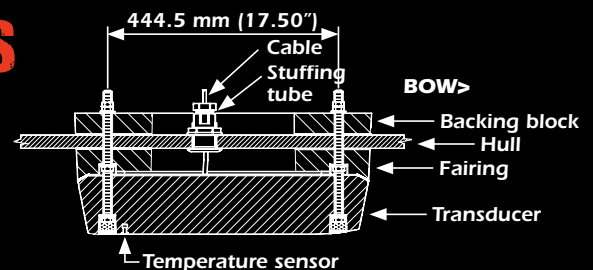
Installing the Transducer
