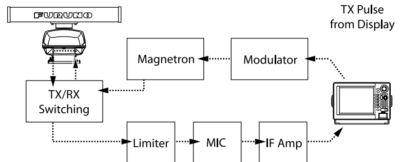
Figure 3 - Circuits and devices of a scanner unit
