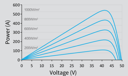
Power-Voltage (540W)
