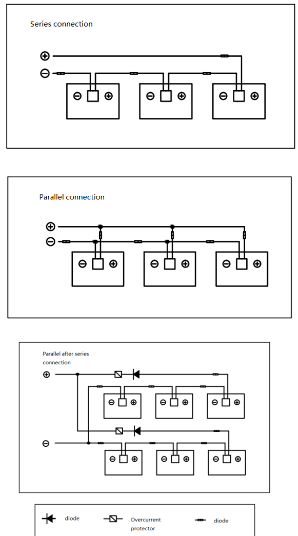
Fig. 17 Schematic diagram of electrical connection
