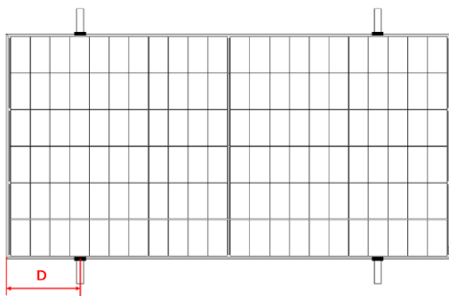
Fig. 4 Rails vertical to the long-side frame
