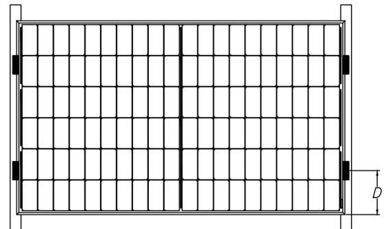
Fig. 5 Rails overlapping the short-side frame
