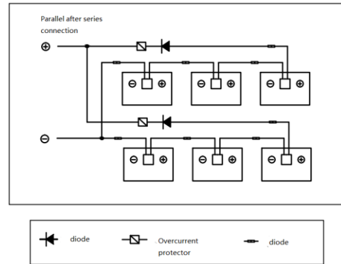
Fig. 17 Schematic diagram of electrical connection
