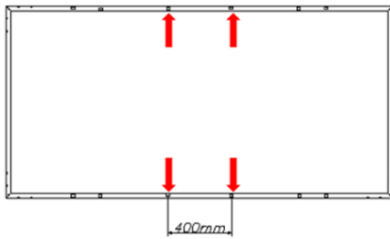
Fig. 9 72cell PV module 400mm spacing bolt installation
