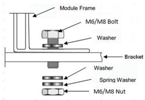
Fig. 10 Diagram of the bolt installation process
