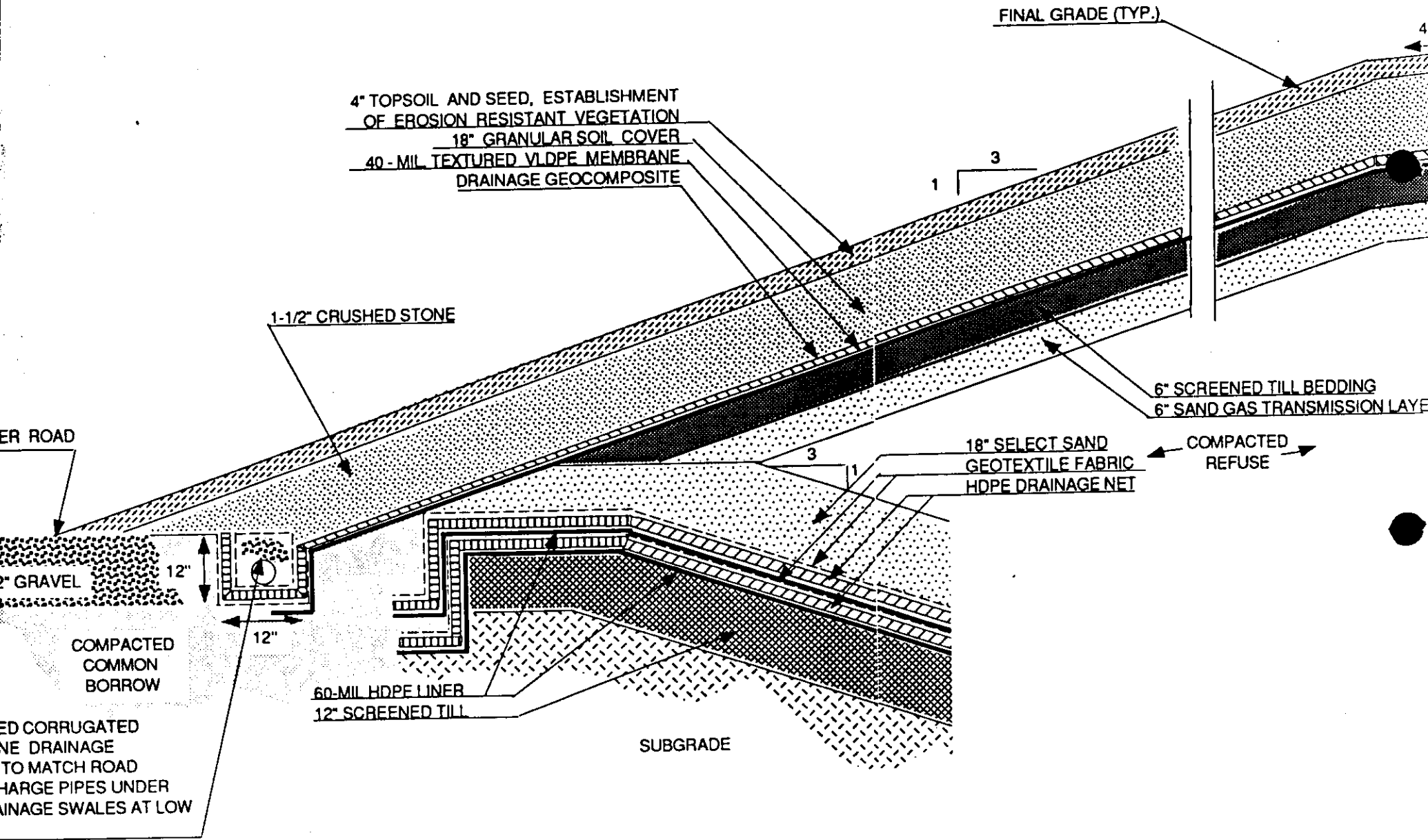
CROSS SECTION - FINAL COVER SYSTEM
