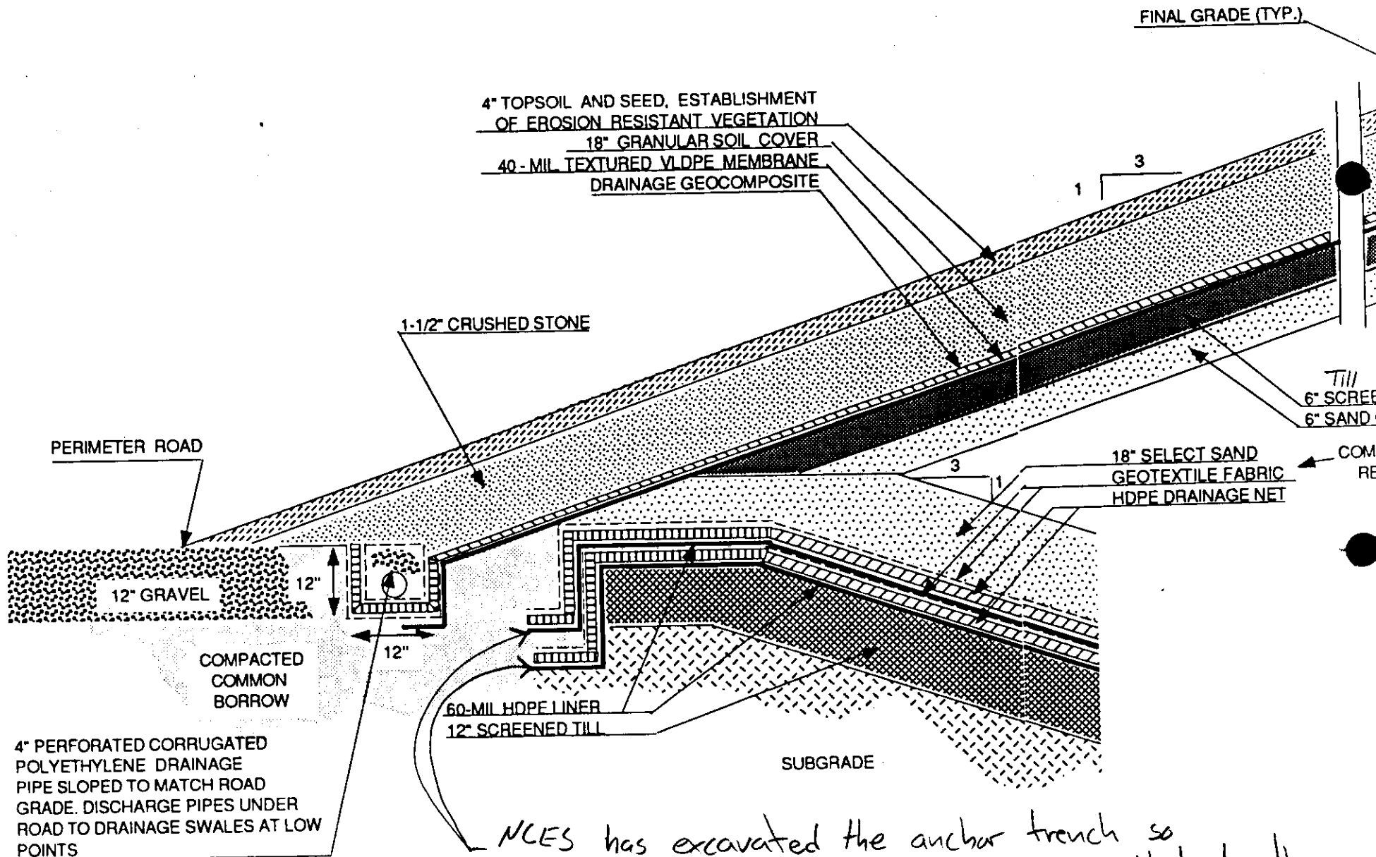
CROSS SECTION - FINAL COVER SYSTEM
