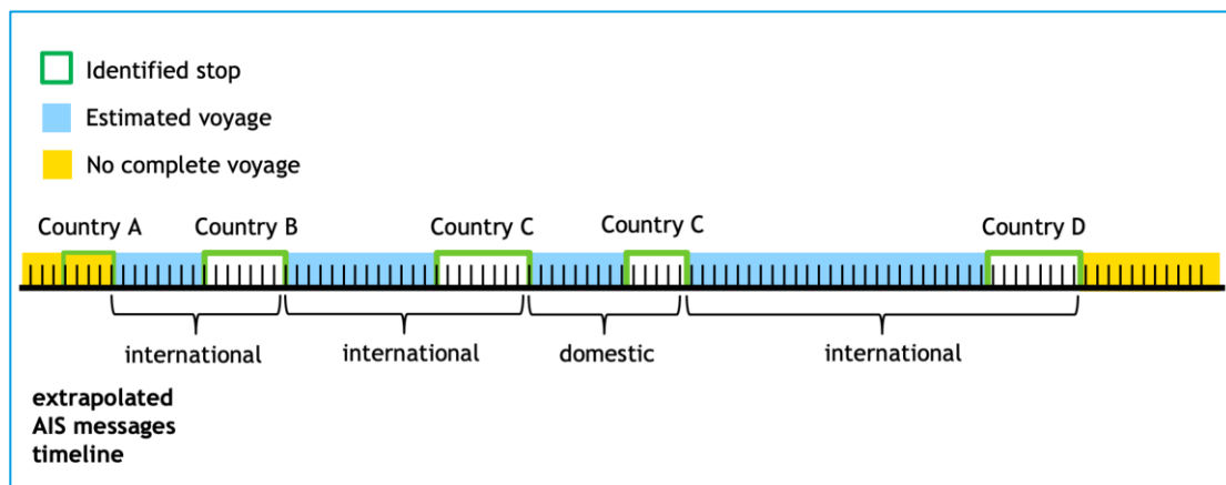
Figure 10 - Allocation of international and domestic nature of shipping according to voyage-based method
