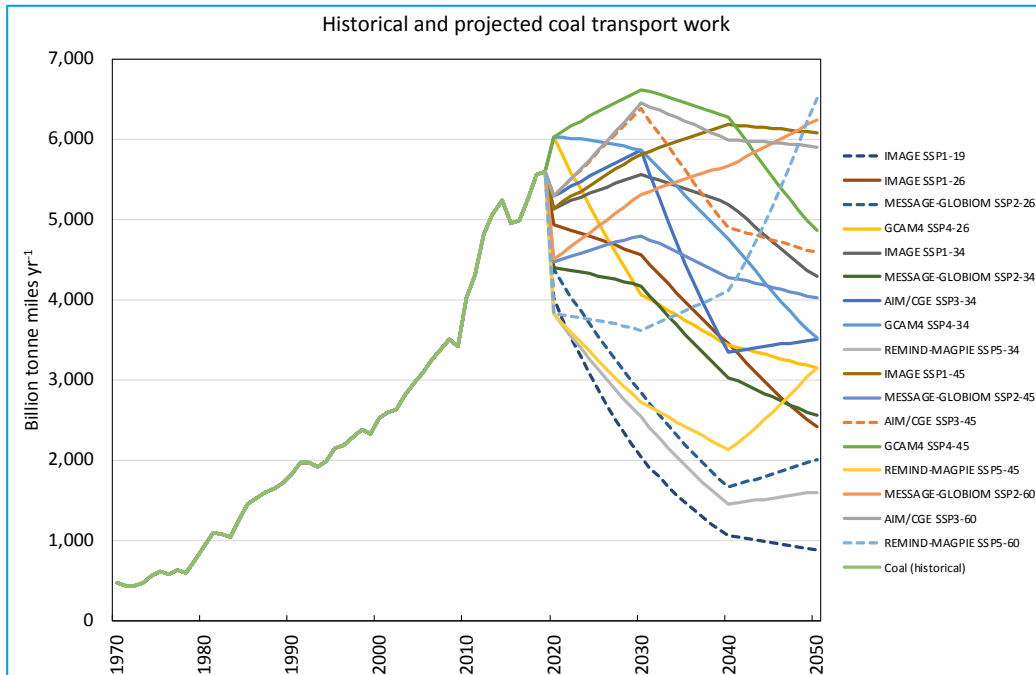
Figure 25 - Historical and projected transport work (109 tonne miles yr-1) to 2050 for coal and oil according to RCP/SSP scenarios
