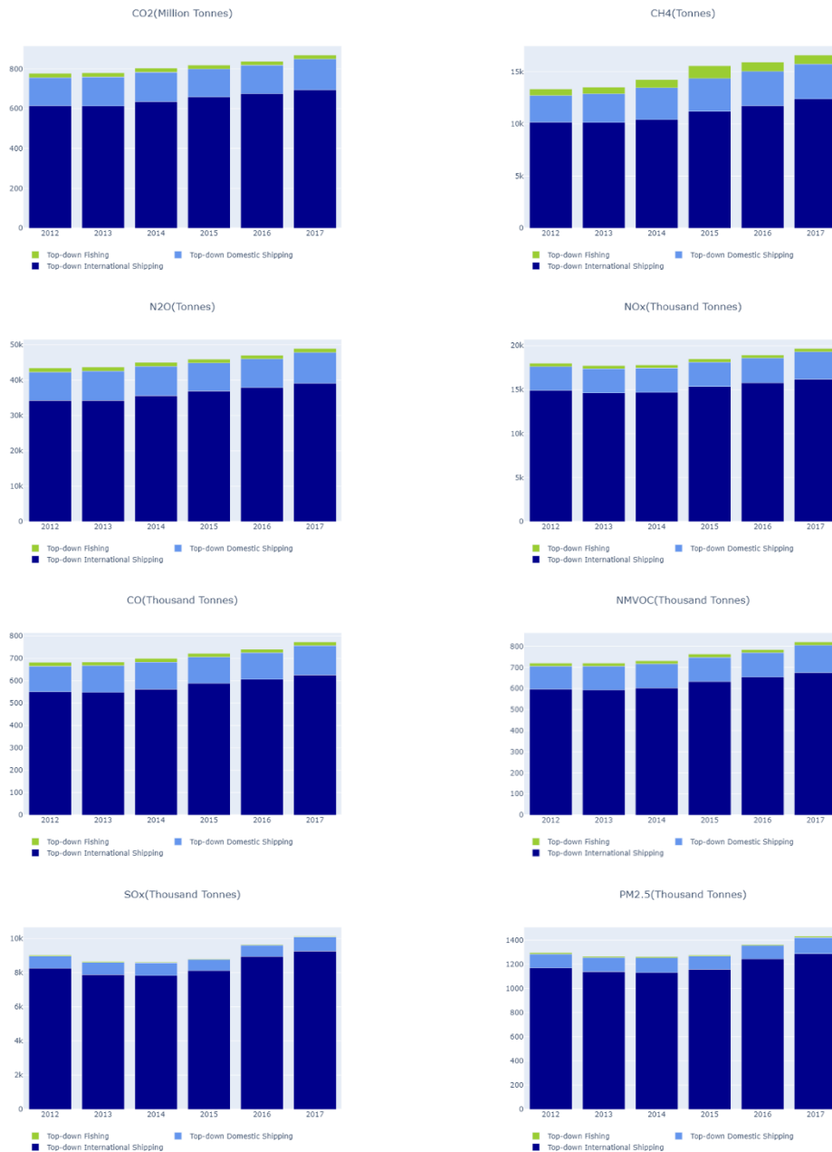
Figure 84 - a) CO 2 , b) CH 4 , c) N 2 O, d) NO x , e) CO, f) NMVOC, g) SO x , h) PM 2.5 , i) PM, h) BC, delineated by international shipping, domestic navigation and fishing
