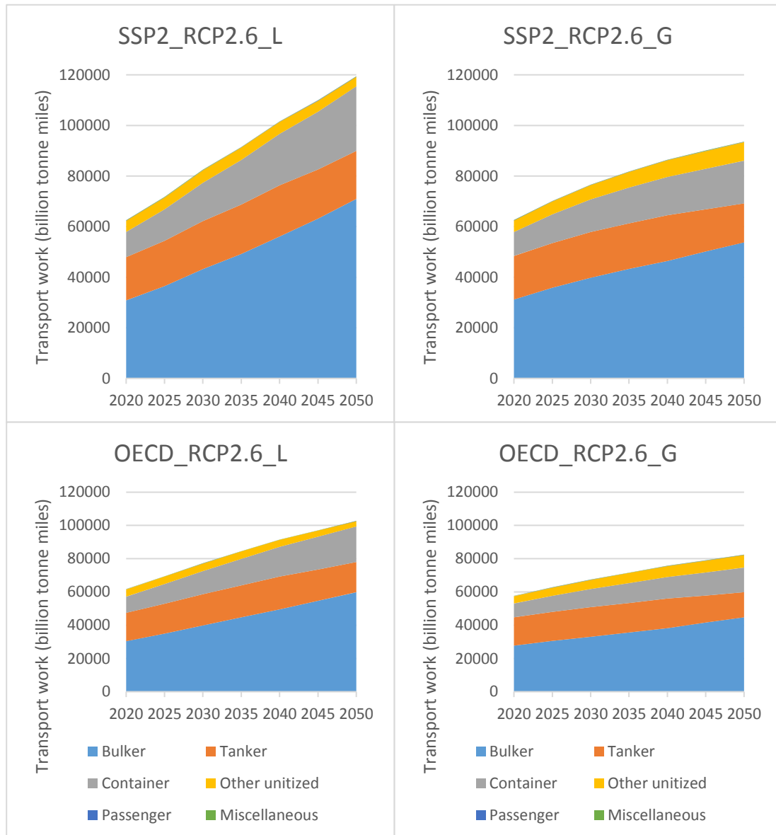
Figure 24 - Transport work projections (billion tonne miles)
