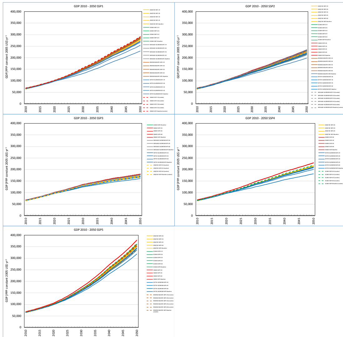
Figure 22 - SSP/RCP combinations by modelling group SSP1 - SSP5
