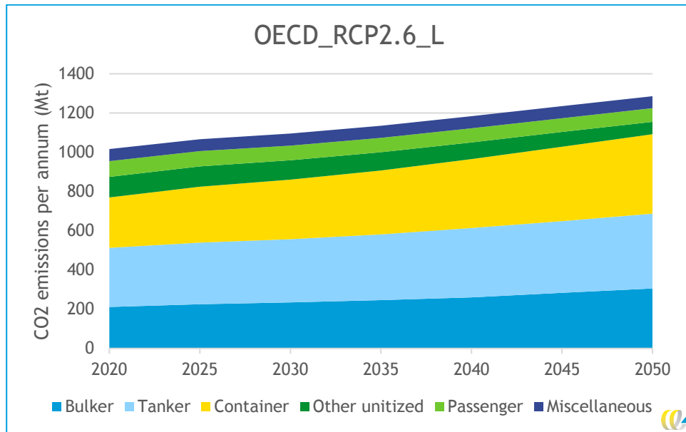
Figure 170 - Emission projections per ship type
