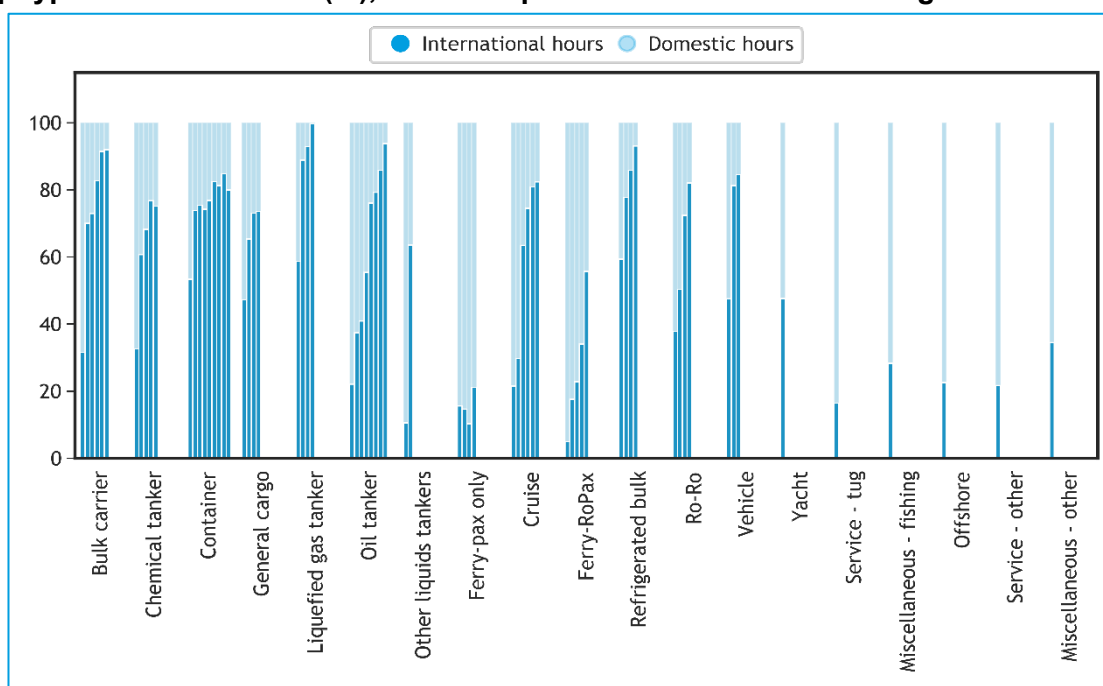
Figure 11 – Proportion of time spent on international and domestic voyages on average by ship type and size in 2018 (%), where ship sizes are order small to large
