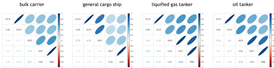
Figure 154 - Correlation between carbon intensity metrics
