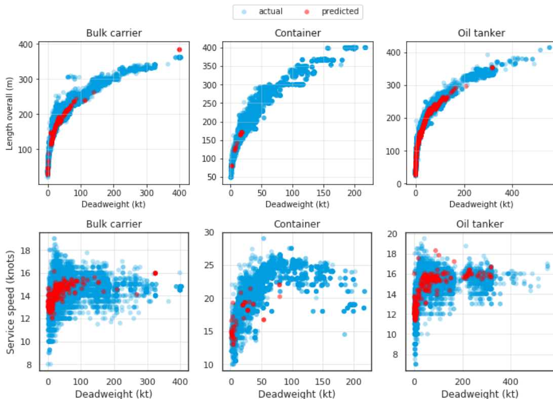
Figure 28 - Example fits when infilling missing technical specification using multilinear regression approach
