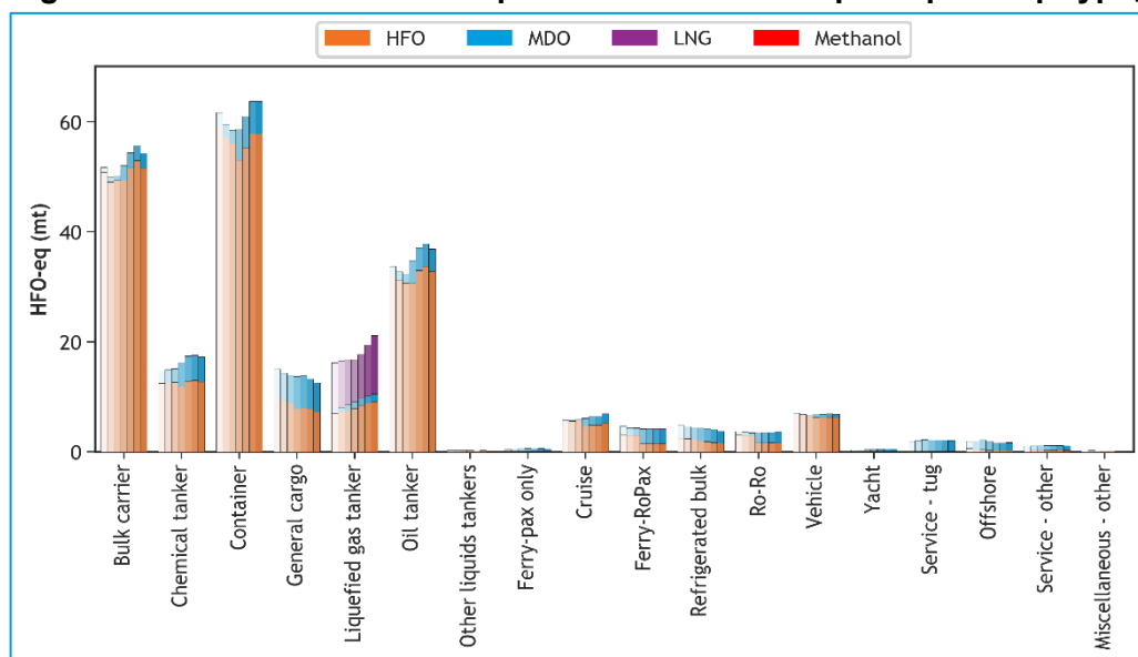
Figure 4 – International HFO-equivalent fuel consumption per ship type, according to
