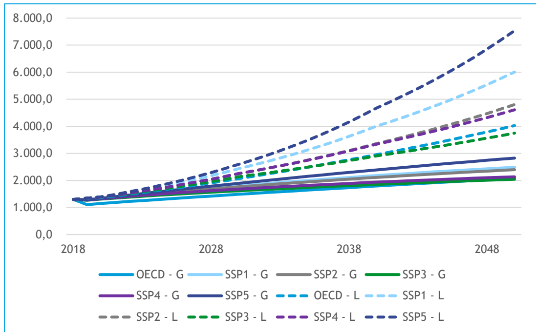
Figure 36 - Transport work Predictions: Logistic (L) Vs gravity model (G) based on Table 3's estimates, 2018-2050, Chemical Tankers
