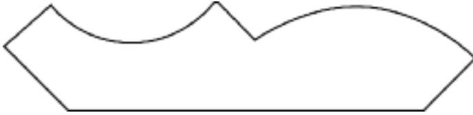
CR 13. 3 15/16" Crown Mould
