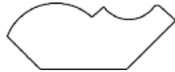
CR 2. 1 3/4" Crown Mould
