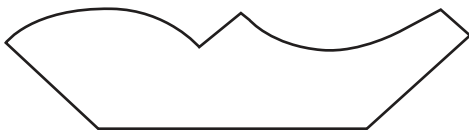
CR 7. 2 5/8" Crown Mould
