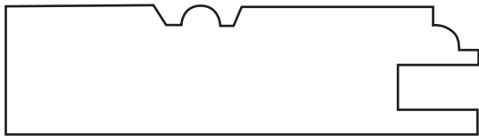
FR 5. 3" Framing
