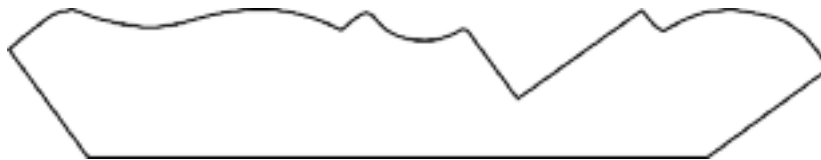
CR 17. 4 1/2" Crown Mould - Roman
