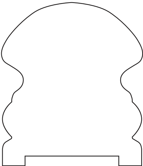
6519 2 5/8" x 3" Hand Rail
