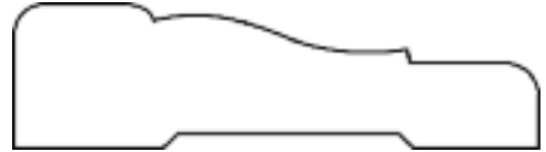
CA 2. 2 1/2" Colonial Casing
