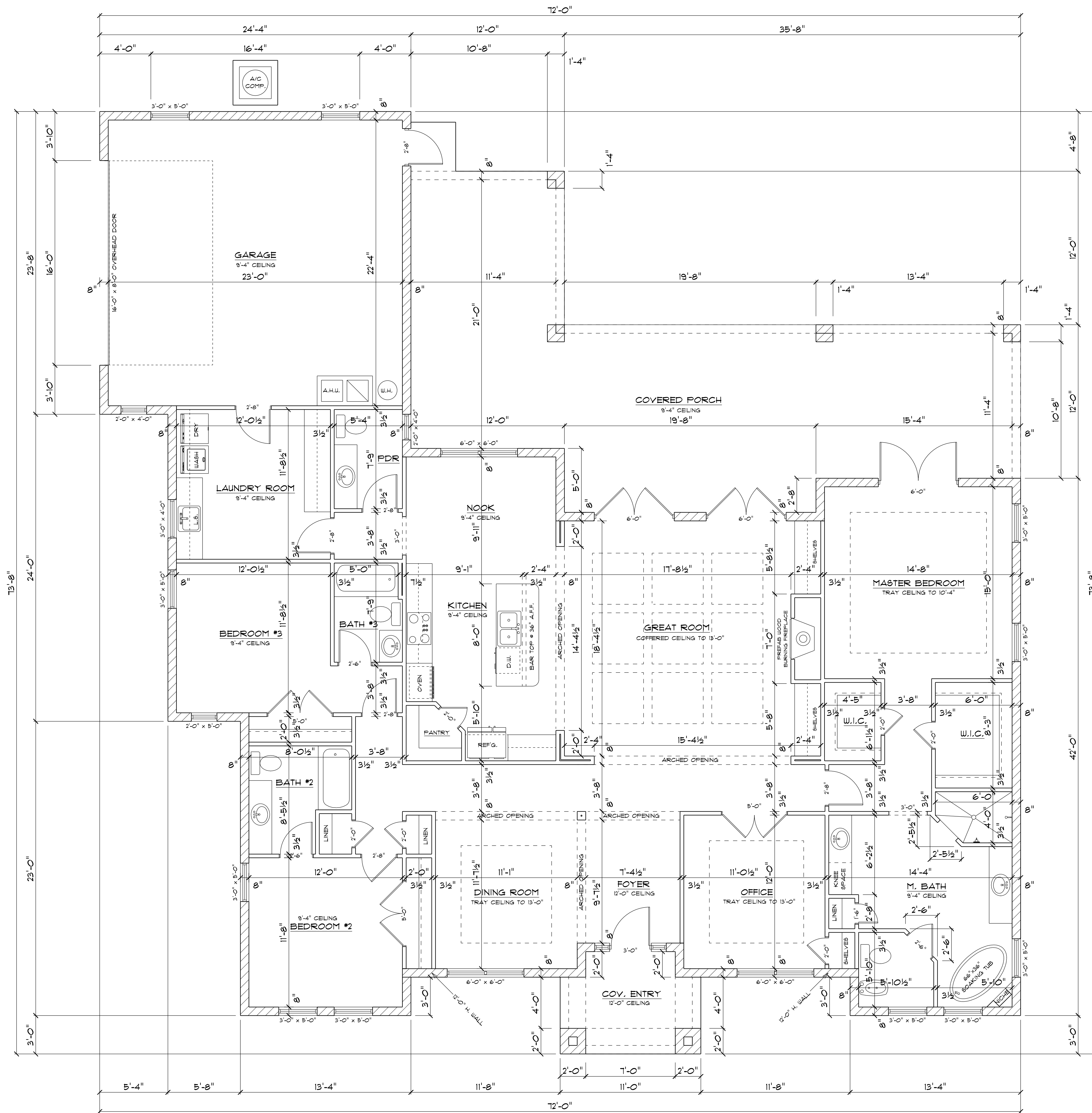
PROPOSED FLOOR PLAN
