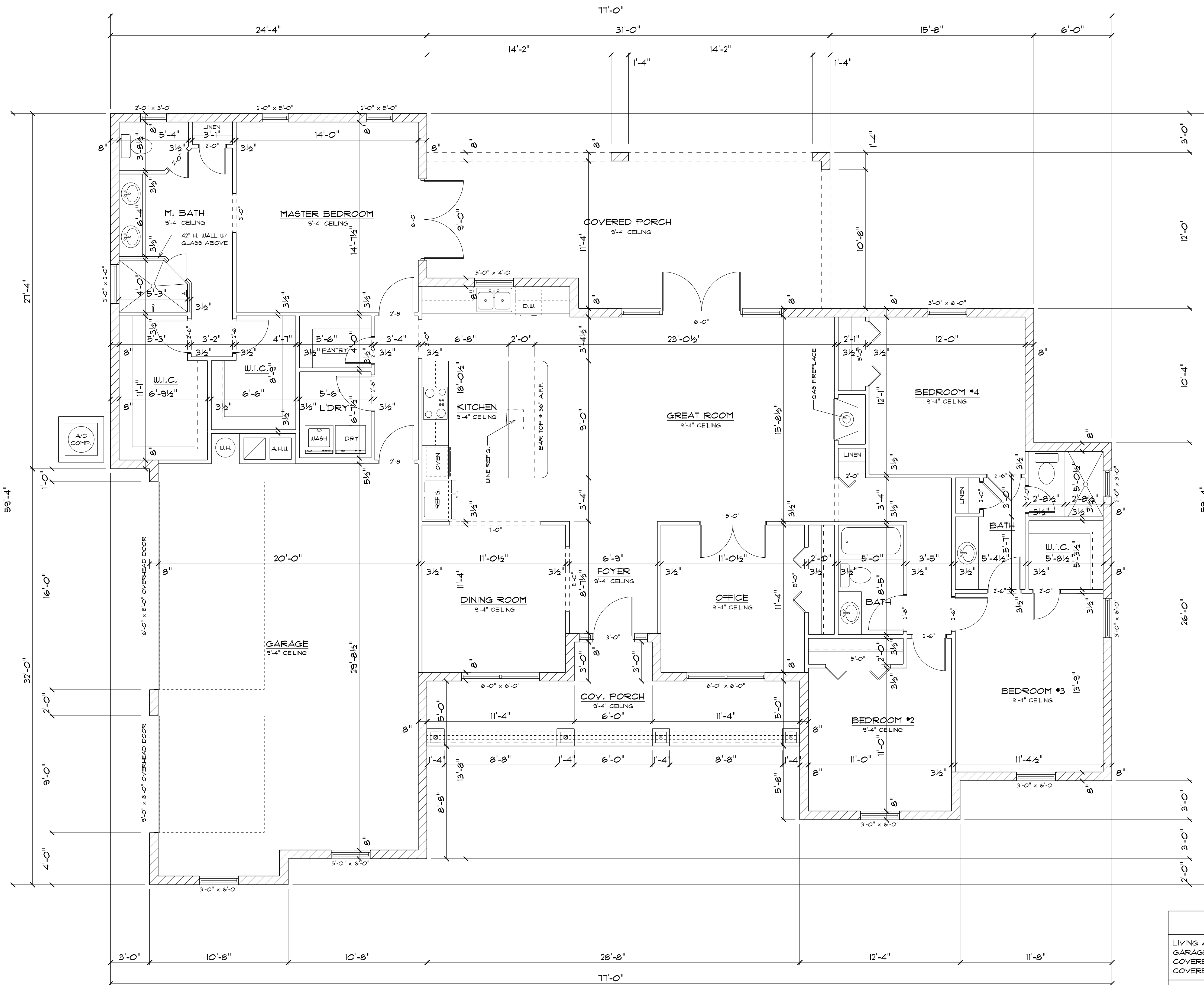
PROPOSED FLOOR PLAN
