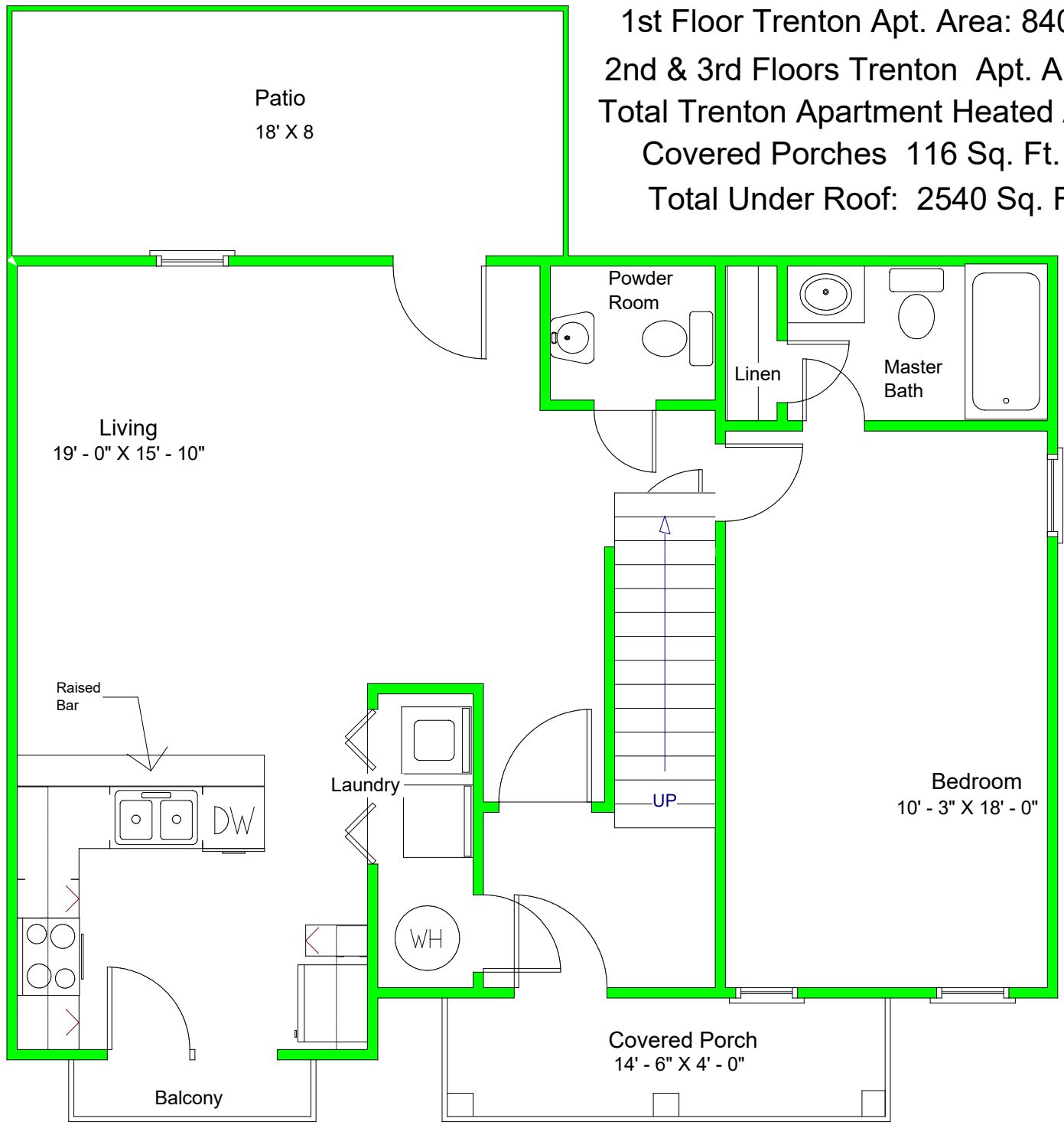
1st Floor (Street Level) of 3 Level Trenton 11+3 Apt. Building
