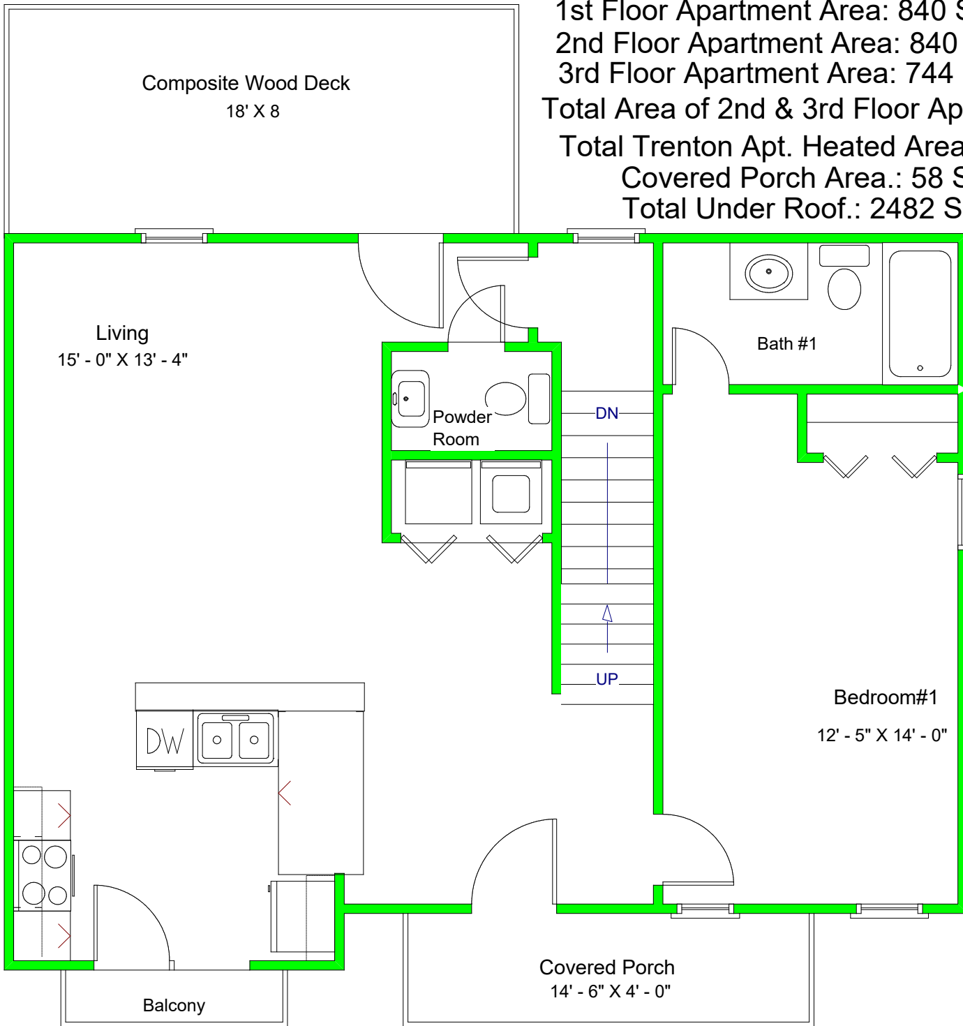
2nd Floor (2nd Level) of 3 Level Trenton 21+3 - 2 Unit Apt. Building
