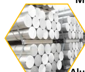
Aluminum
