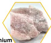
Lithium
