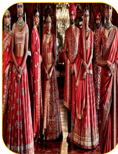
Palladium
