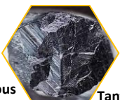
Tantalum
