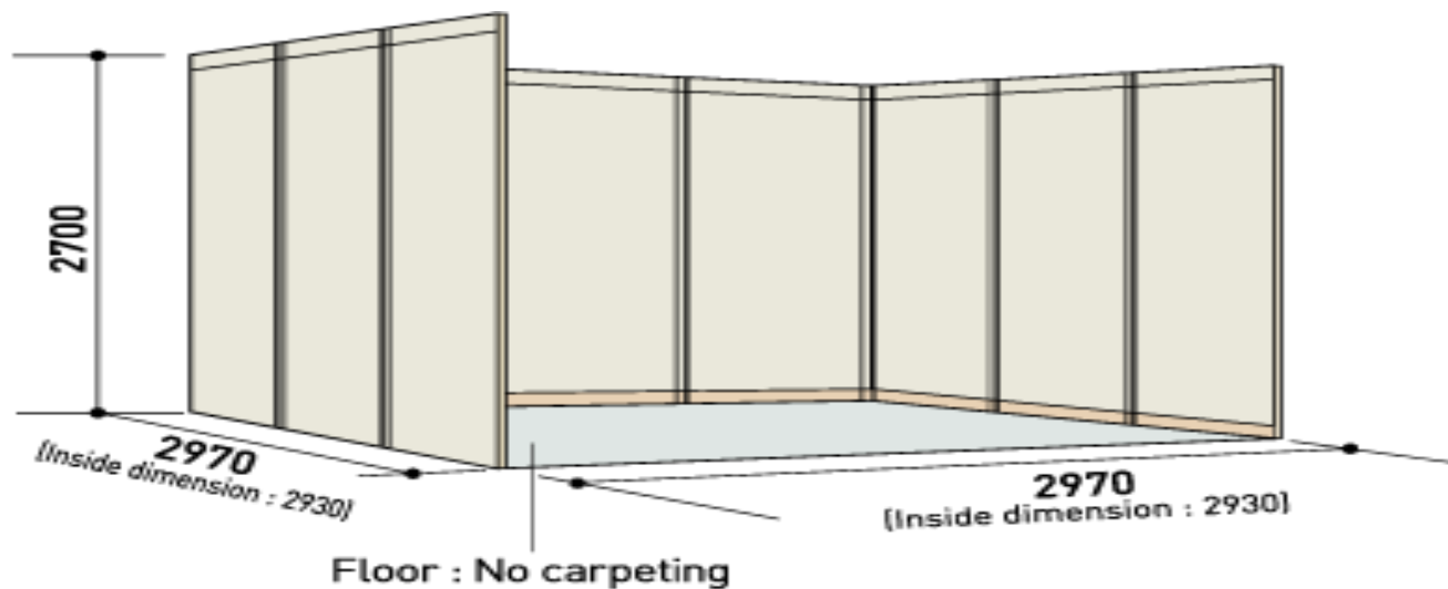
System wall panel (octanorm system)
