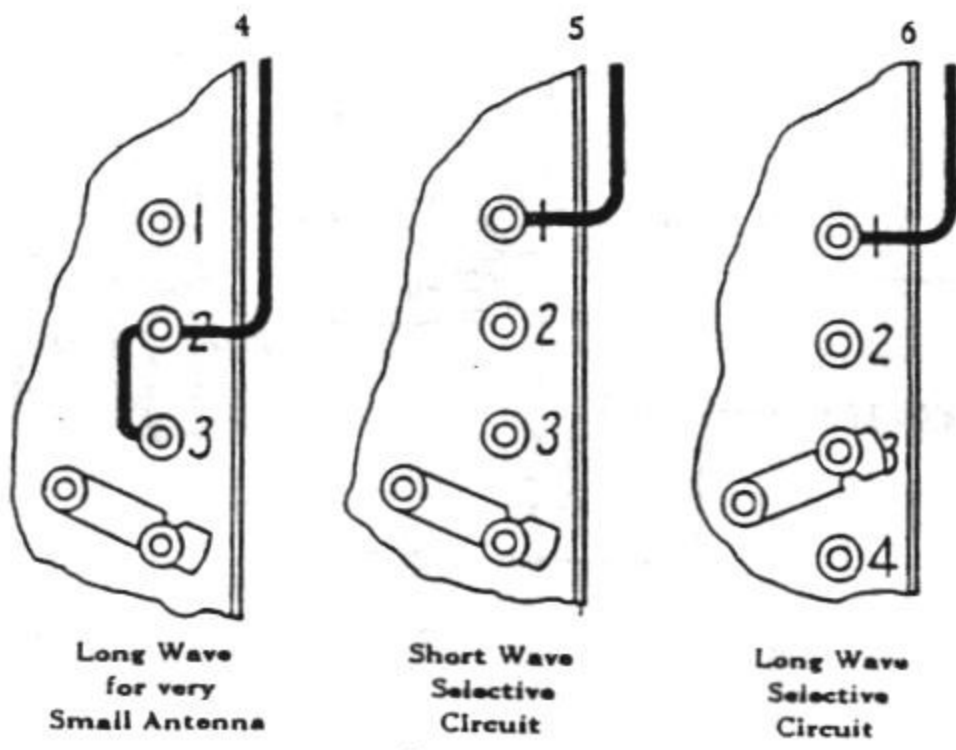
Fig. 3—Showing Antenna Connections to Different Binding Posts
