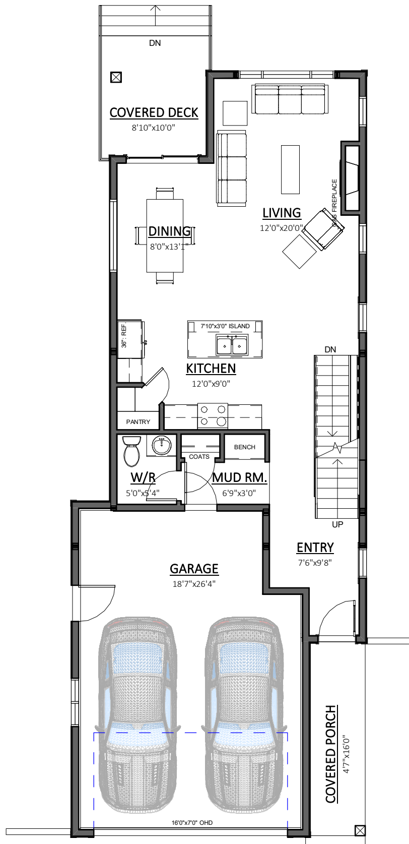
I MAIN FLOOR PLAN MI 1/8" = 1'-0" 782 SQ. FT.
