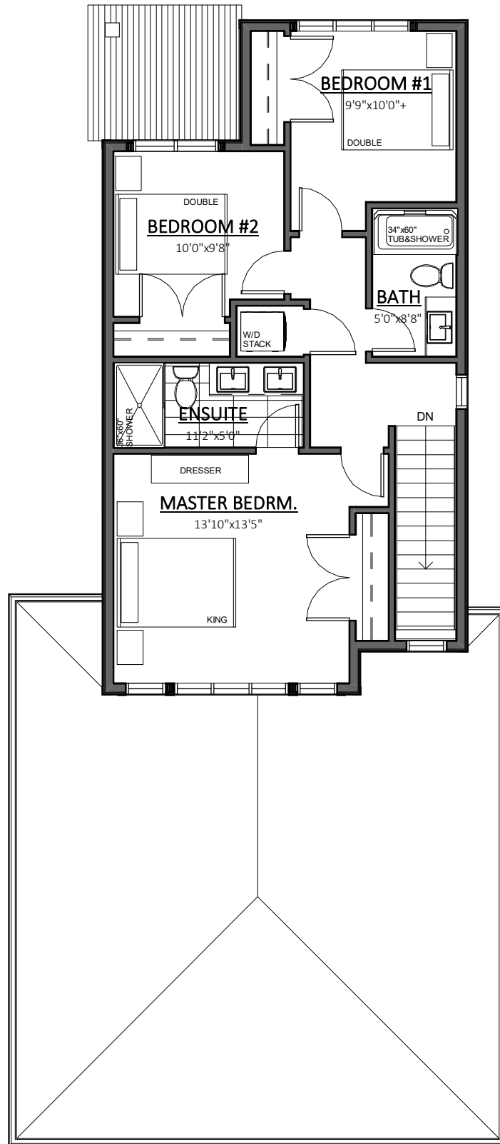
1 UPPER FLOOR PLAN M2 1/8" = 1'-0" 747 SQ.FT.
