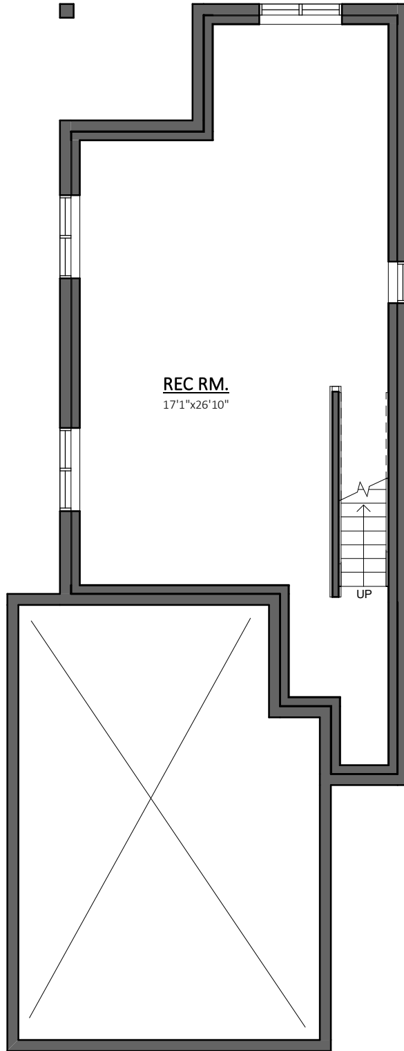
1 BASEMENT PLAN M3 1/8" = 1'-0"
