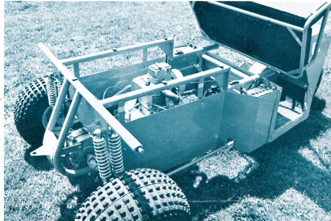
Bed removes in 3 minutes (with just 2 bolts) . . . all parts readily accessible for fast, easy service and maintenance.
