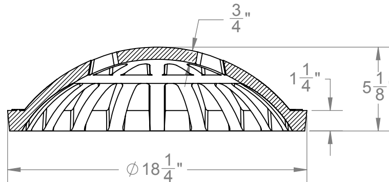
SECTION AL-AL SCALE 1 : 6
