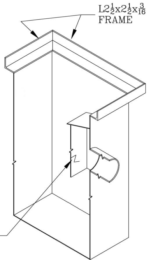
ISOMETRIC SECTION
