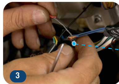
Connect the red wire to the vehicle constant power wire.
