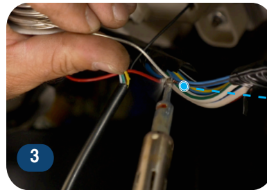
Solder wires to ensure a good connection.
