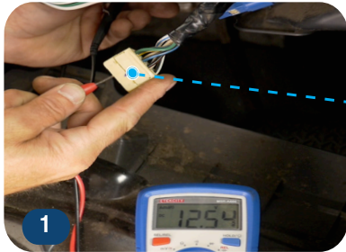
Voltmeter testing power output.
