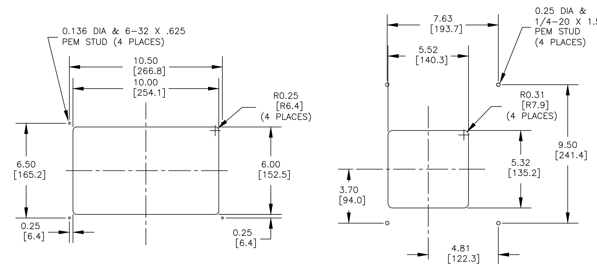
DETAIL A -1 (FOR TYPE 1)
