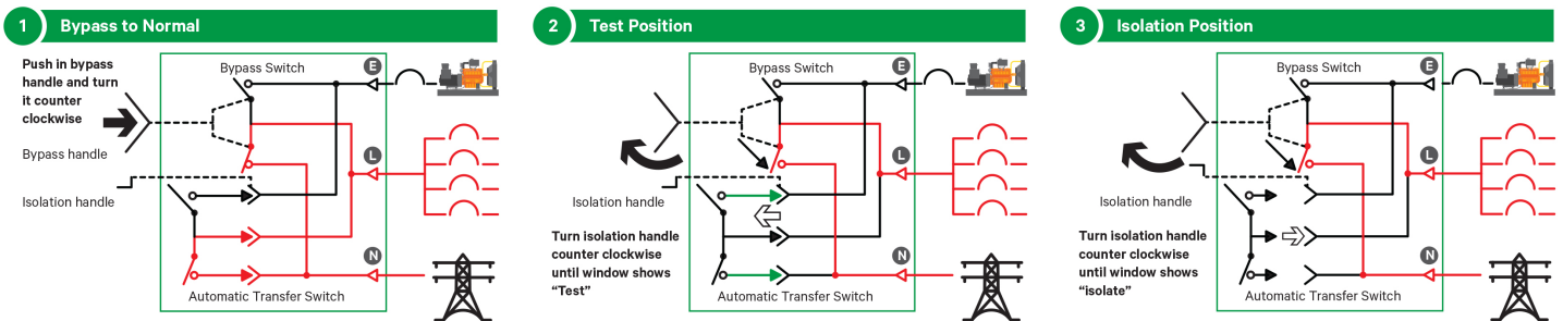
Figure 9: ASCO Bypass-Isolation Operating Sequence
