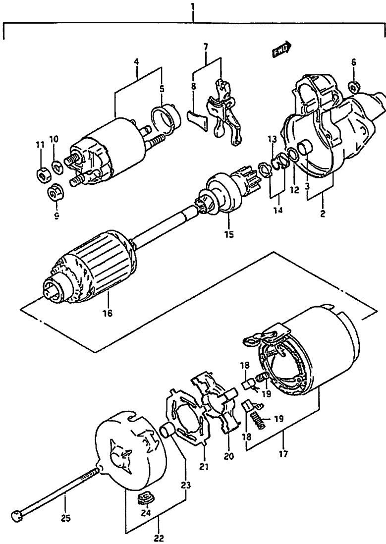
Fig: 72 Electrical Components Starter Motor: Type 2
