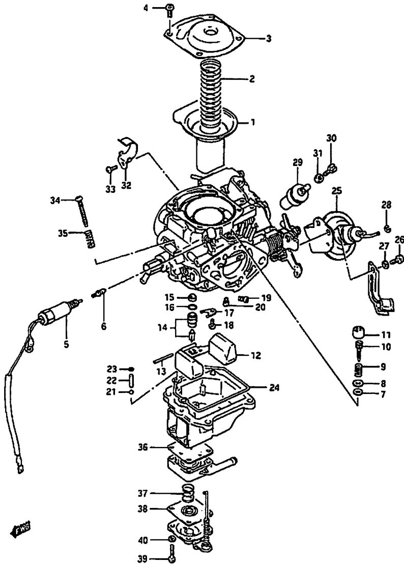
Fig: 16 Engine Group Carburetor Components
