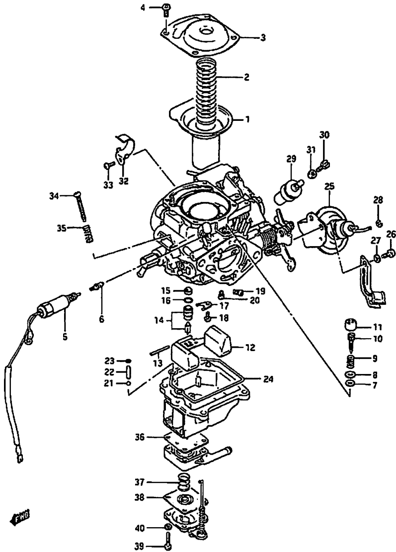
Fig: 16 Engine Group Carburetor Components
