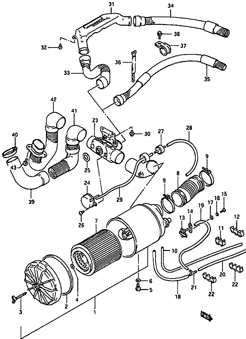
Fig: 22 Engine Group Air Cleaner: Every Van: Standard
