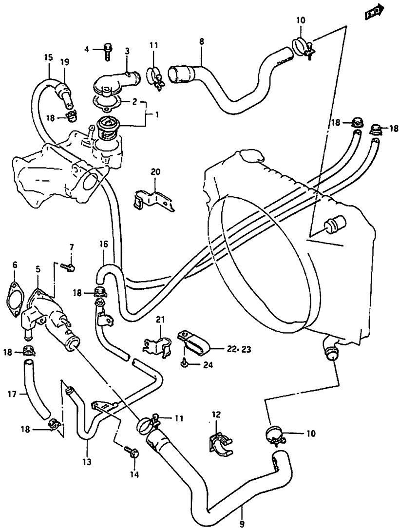
Fig: 41 Cooling & Emission System Components Water Hose & Components: Standard
