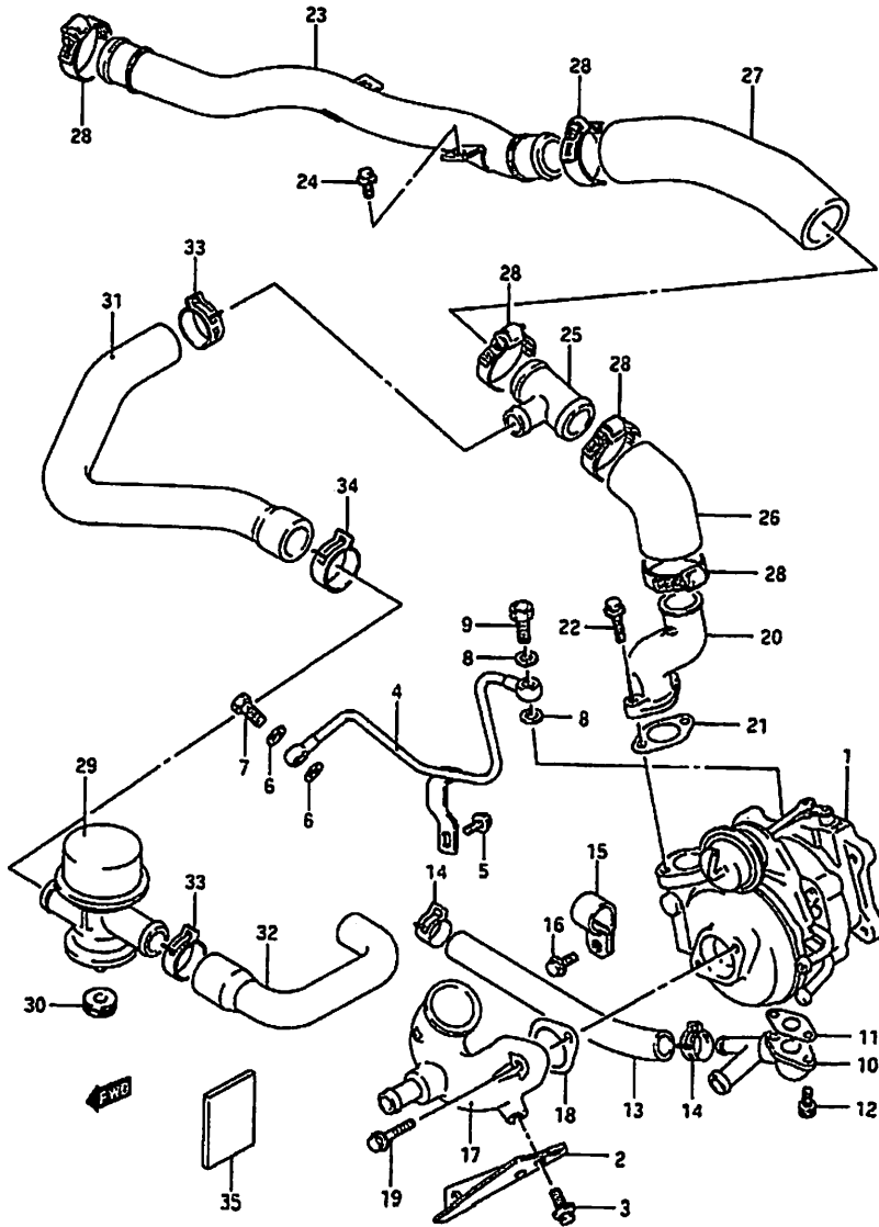
Fig: 30 Engine Group Turbocharger System: Type 2.
