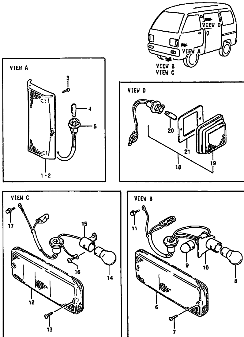
Fig: 85 Electrical Components Front Turn Signal & Running Lamps
