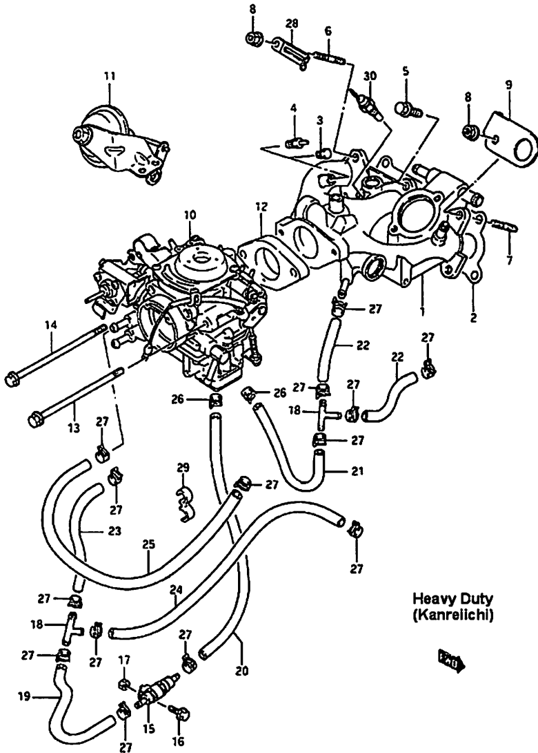
Fig: 14 Engine Group Intake Manifold: Carbureted: Type 2: Heavy Duty
