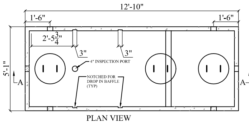
PLAN VIEW
