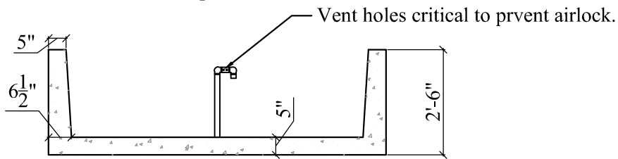
Section View
