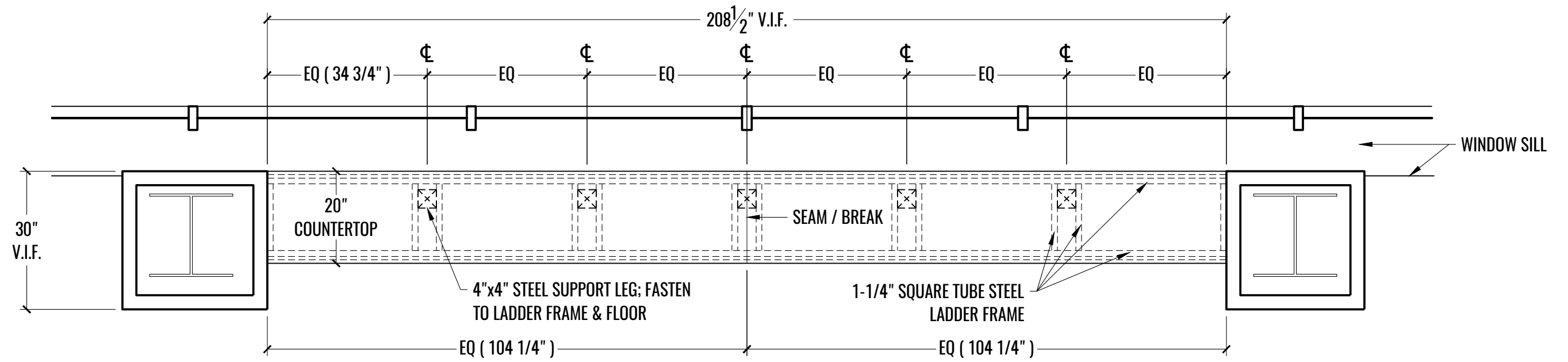
1 PLAN: MEETING AREA 630 11 SCALE: 1/2" = 1'-0"
