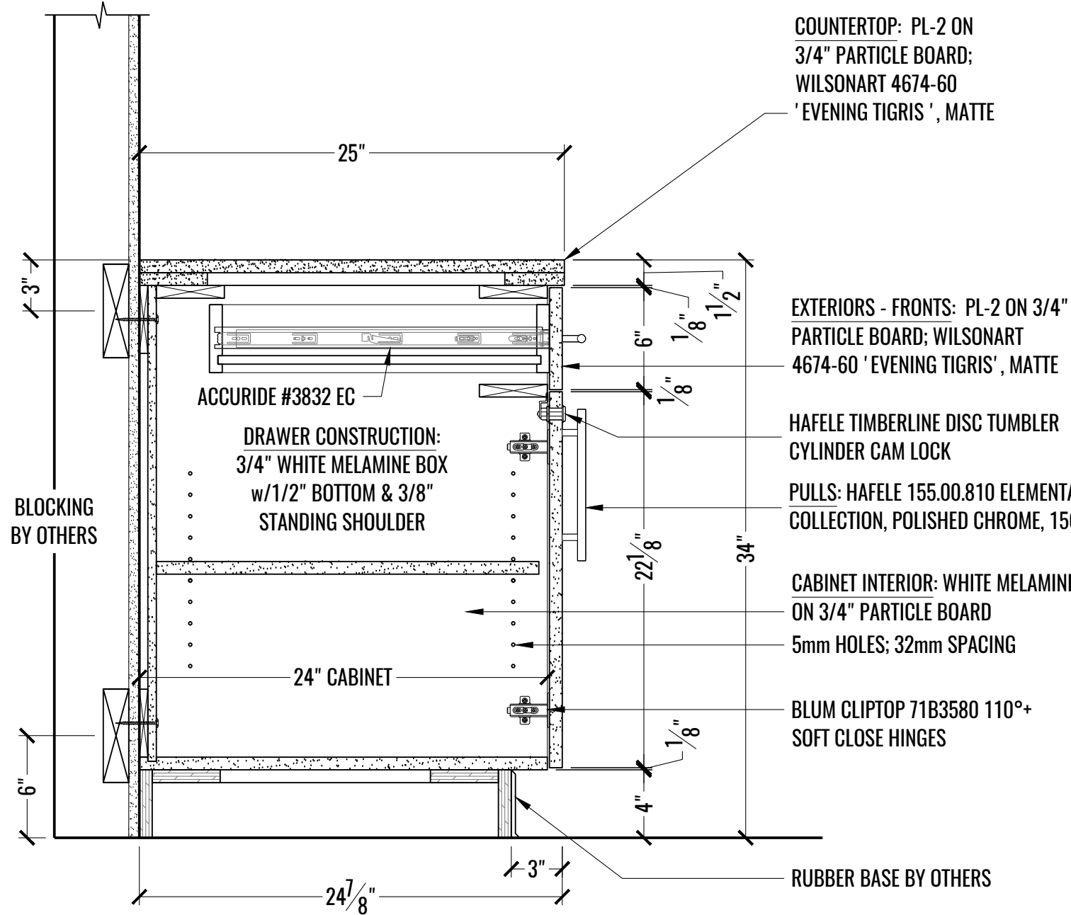
1 SECTION: COPY / PRINT 605 TYP. BASE CABINET C SCALE: 1-1/2" = 1'-0"
