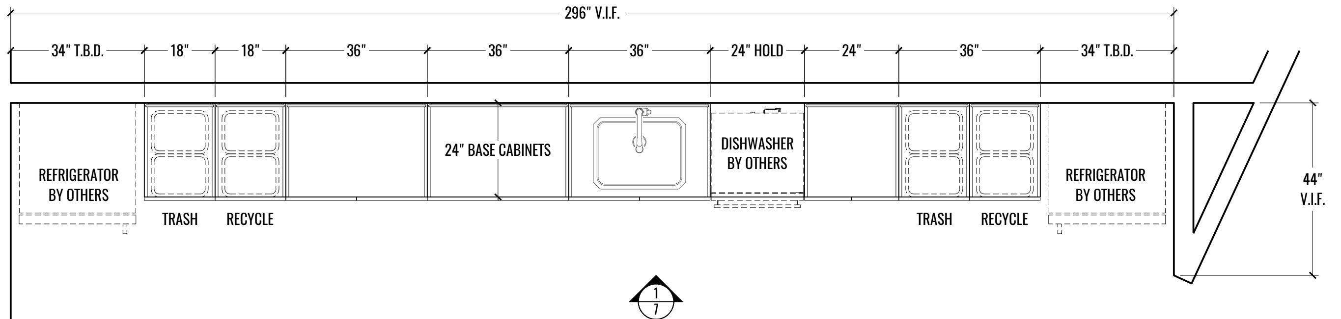
2 PLAN: KITCHENETTE 603 BASE CABINETS 6 SCALE: 1/2" = 1'-0"
