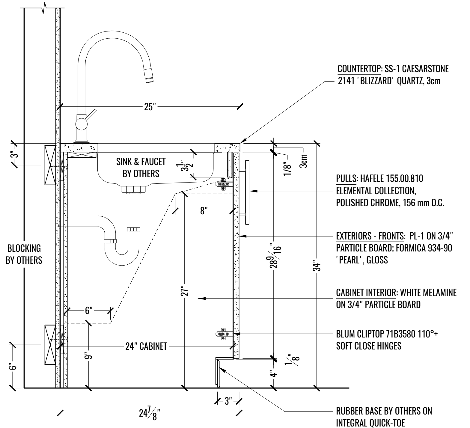
2 SECTION: KITCHENETTE 603 SINK BASE CABINET E SCALE: 1-1/2" = 1'-0"
