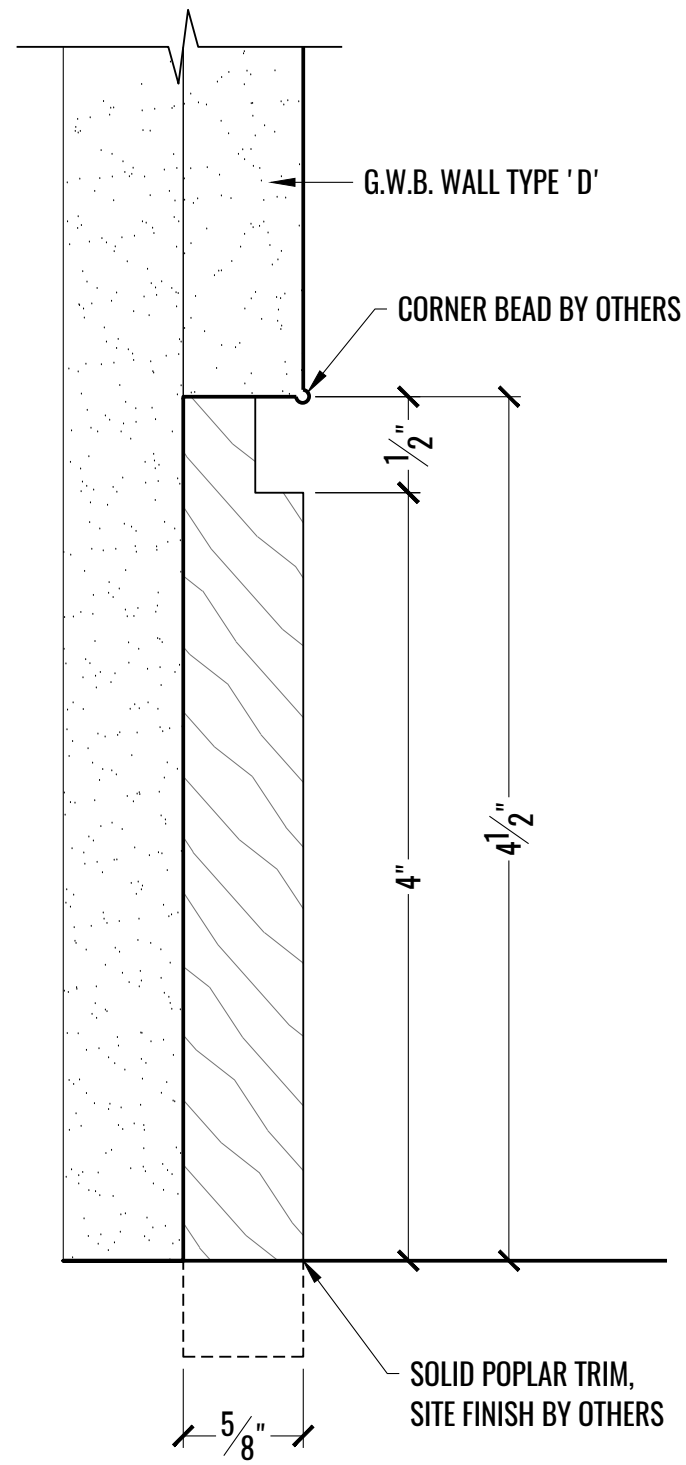
2 A DETAIL: ELEVATOR LOBBY BASE SCALE: FULL
