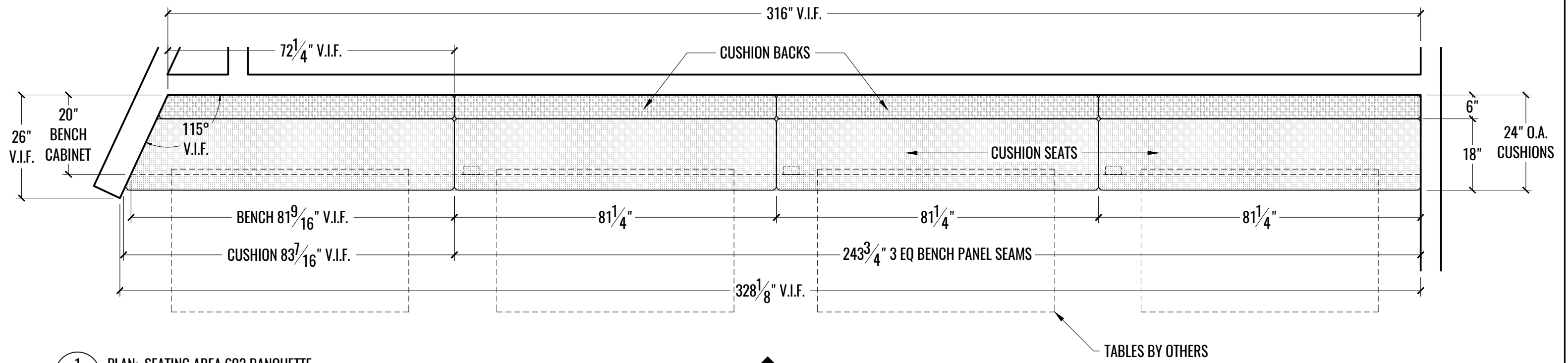
1 PLAN: SEATING AREA 602 BANQUETTE 8 SCALE: 1/2" = 1'-0"
