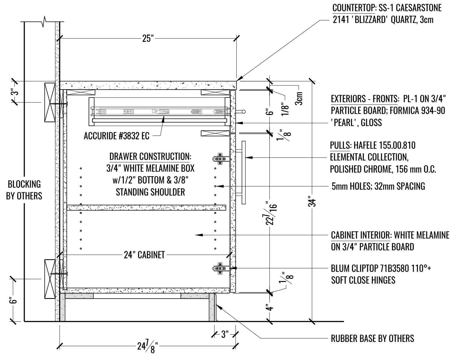
2 SECTION: KITCHENETTE 603 TYP. BASE CABINET F SCALE: 1-1/2" = 1'-0"
