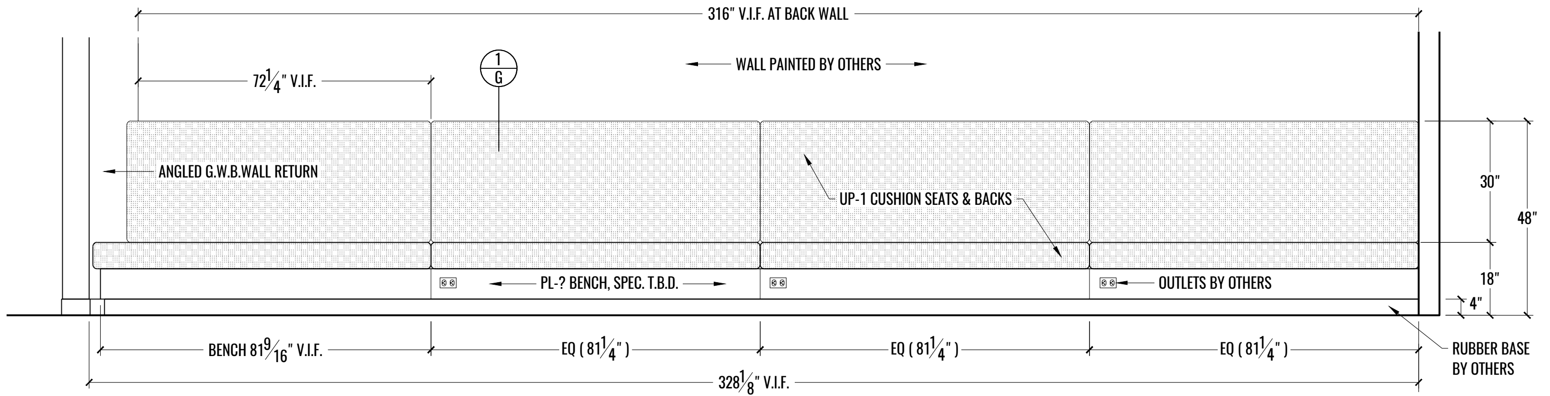
2 ELEVATION: SEATING AREA 602 BANQUETTE 8 SCALE: 1/2" = 1'-0"
