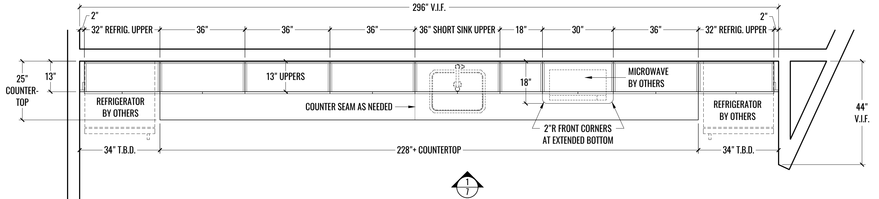
1 PLAN: KITCHENETTE 603 UPPER CABINETS 6 SCALE: 1/2" = 1'-0"
