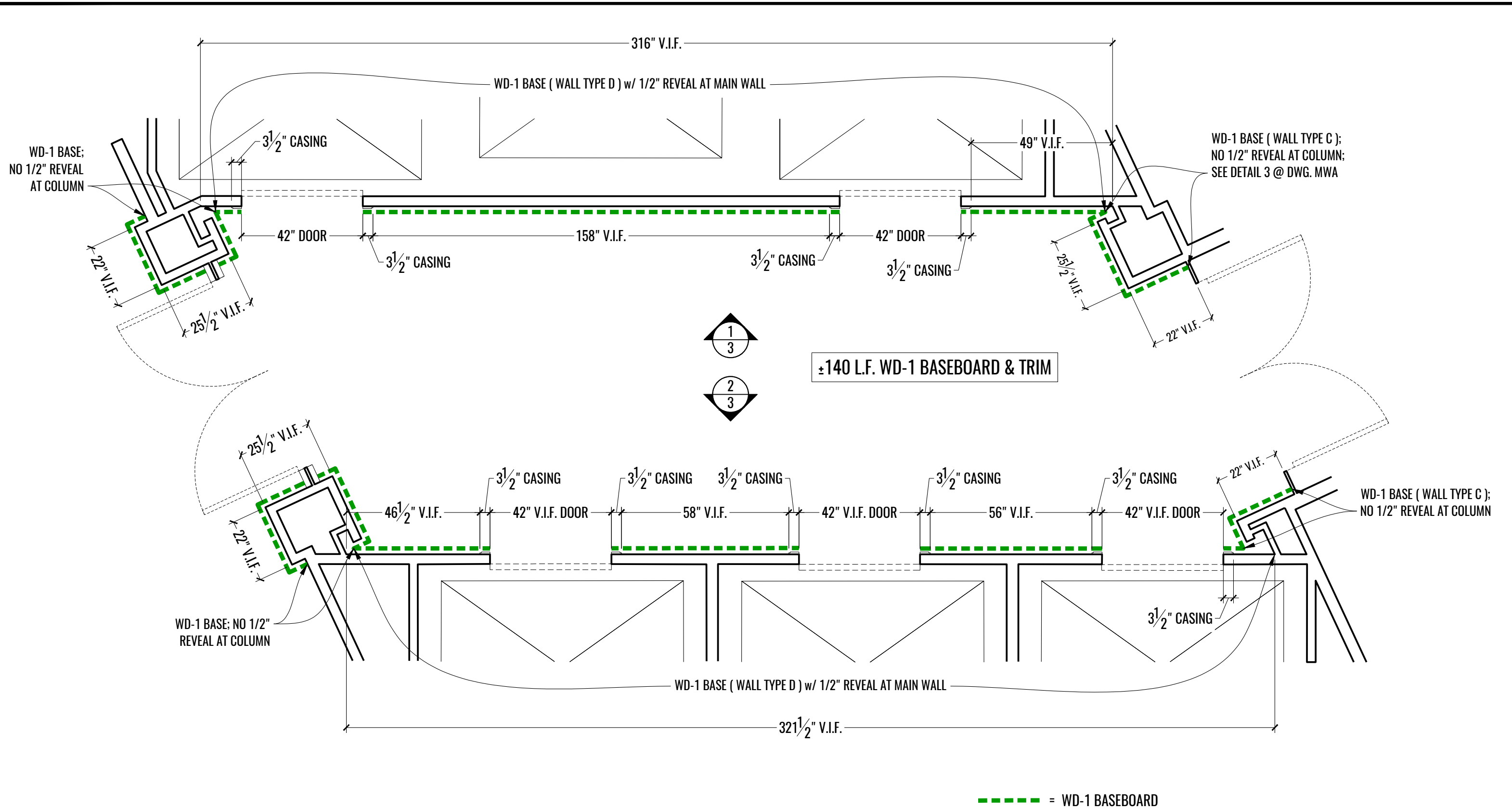
1 PLAN: ELEVATOR LOBBY BASEBOARD & TRIM 2 SCALE: 3/8" = 1'-0"
