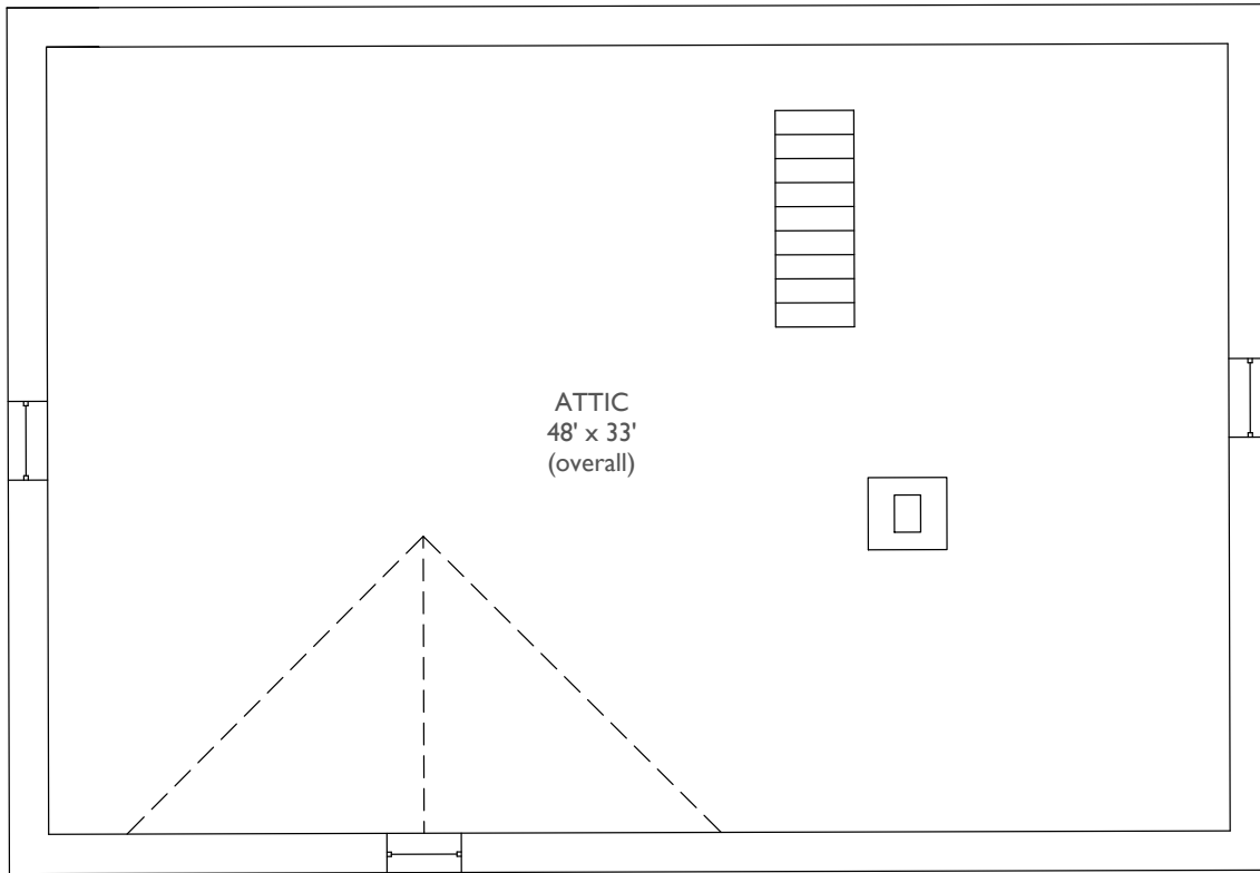
ATTIC PLAN
